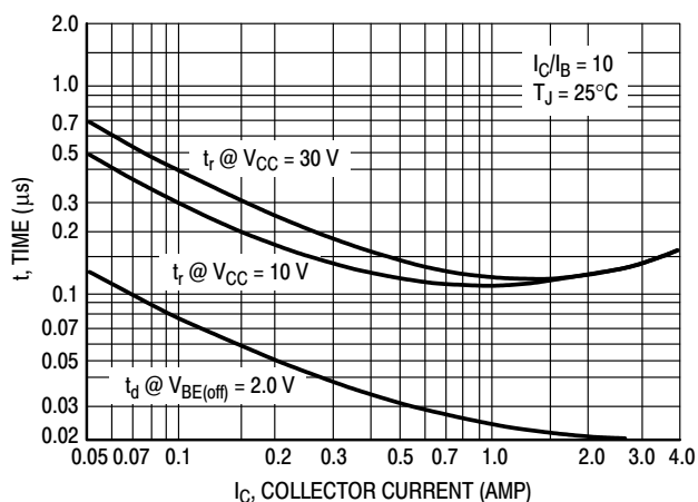
Figure 9. Turn-On Time
