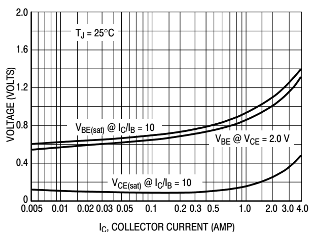
Figure 3. "On" Voltage
