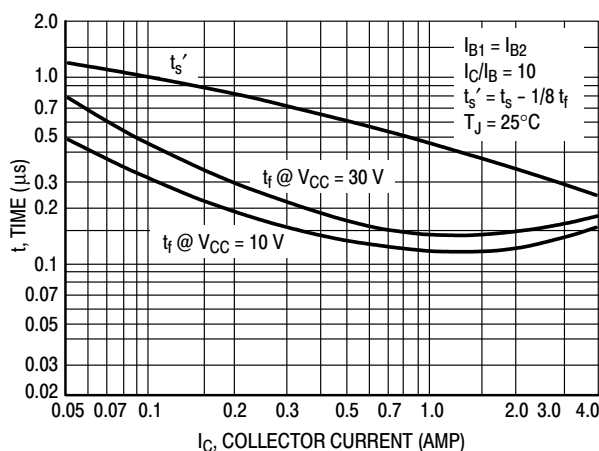
Figure 10. Turn-Off Time
