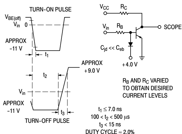
Figure 7. Switching Time Equivalent Test Circuit
