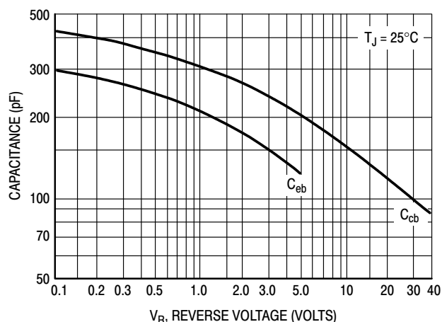
Figure 8. Capacitance
