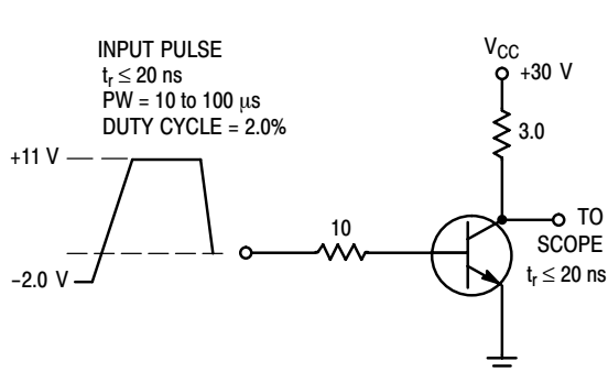
Figure 2. Turn-On time
