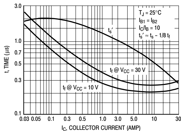
Figure 8. Turn-Off Time
