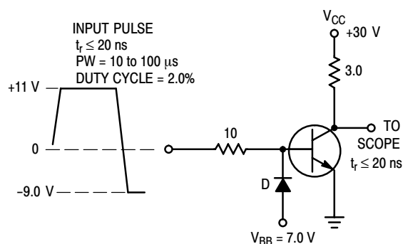
Figure 3. Turn-Off time
