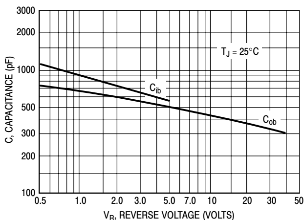
Figure 6. Capacitance versus Voltage
