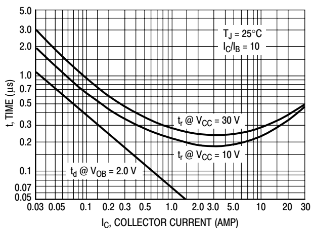
Figure 7. Turn-On Time
