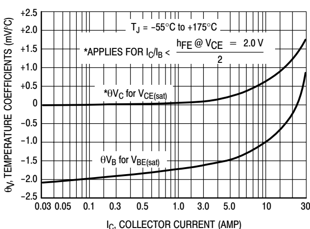
Figure 14. Temperature Coefficients
