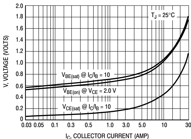
Figure 12. "On" Voltages
