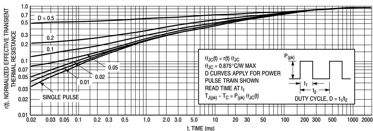
Figure 4. Thermal Response
