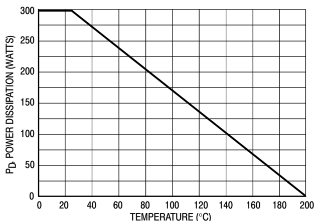
Figure 1. Power Derating
