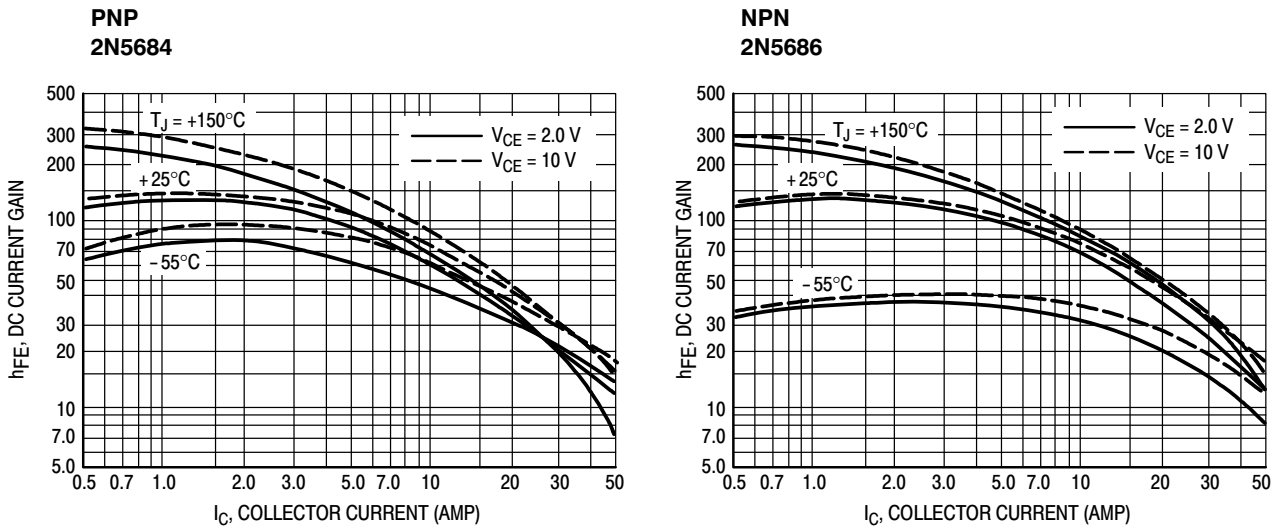
Figure 8. DC Current Gain
