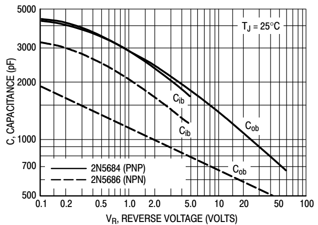
Figure 7. Capacitance
