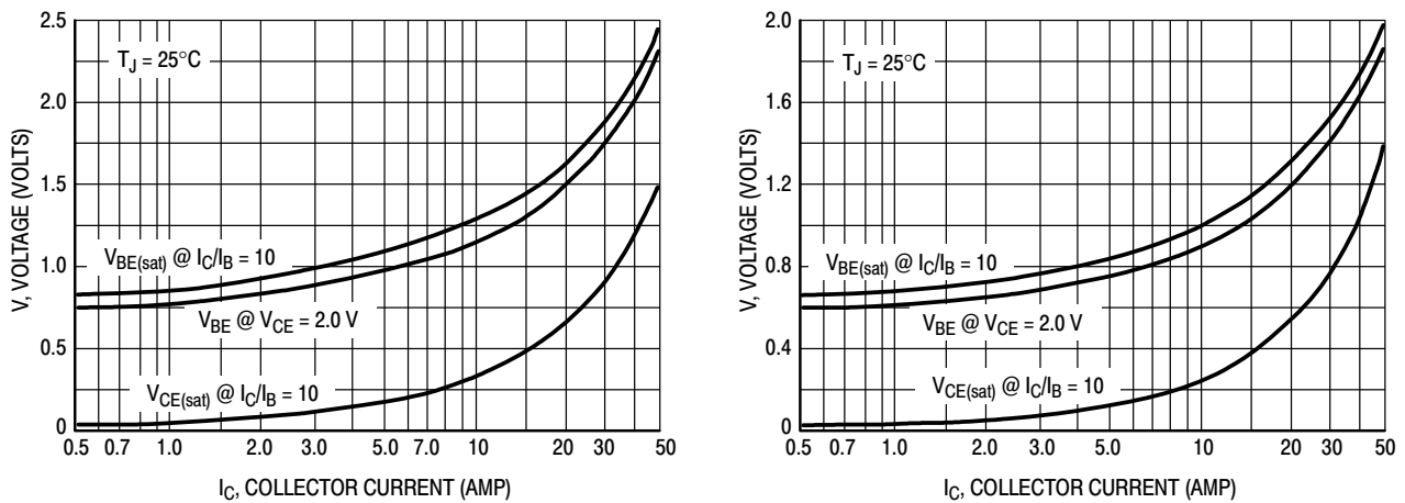
Figure 10. "On" Voltages
