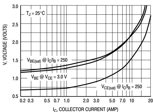
Figure 10. "On" Voltages
