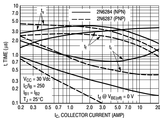
Figure 3. Switching Times
