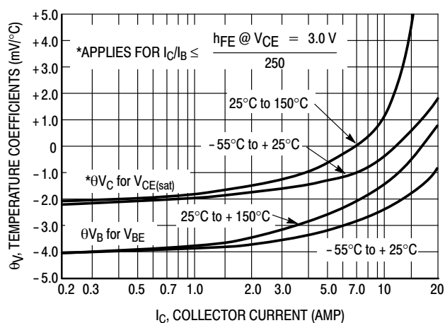
Figure 11. Temperature Coefficients
