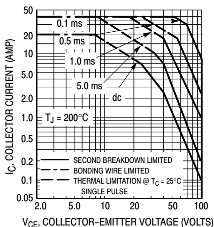
Figure 5. 2N6284, 2N6287
