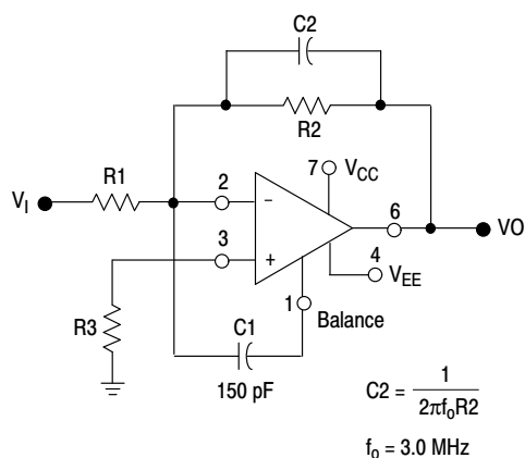
Figure 15. Feedforward Compensation
