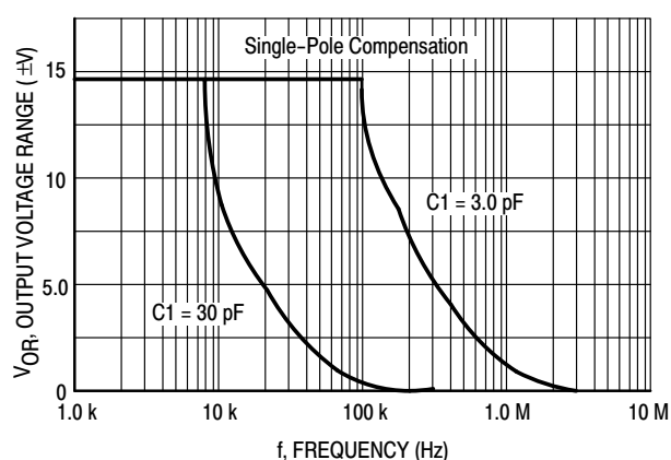
Figure 9. Large Signal Frequency Response
