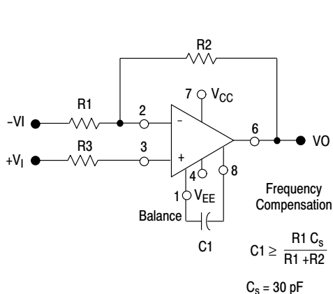
Figure 14. Single-Pole Compensation
