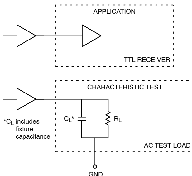
Figure 3. TTL Output Loading Used for Device Evaluation
