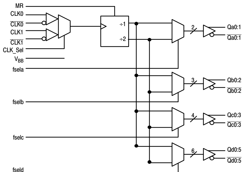
Figure 2. Logic Diagram
