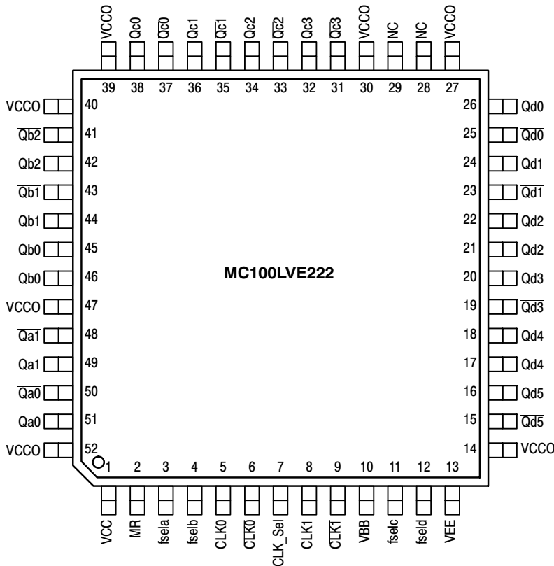
Figure 1. Pinout Assignment (Top View)
