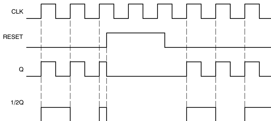
Figure 3. Timing Diagram
