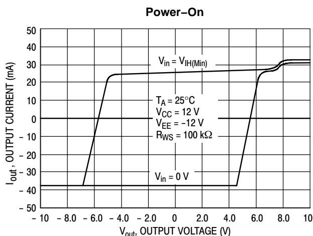
Figure 5. Output Current versus Output Voltage
