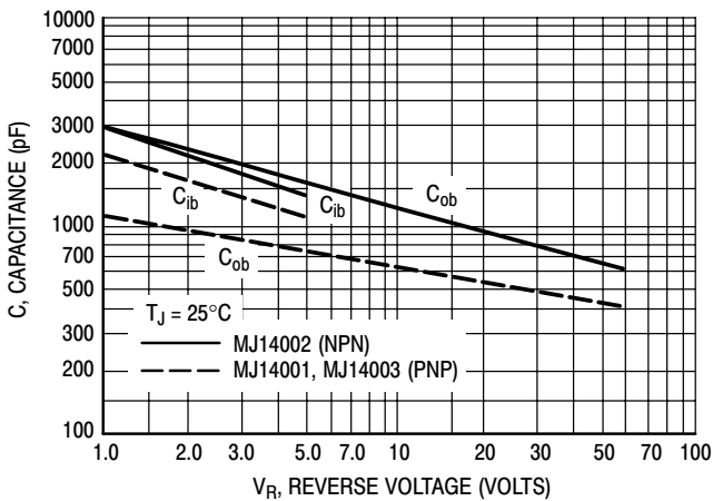
Figure 11. Capacitance Variation
