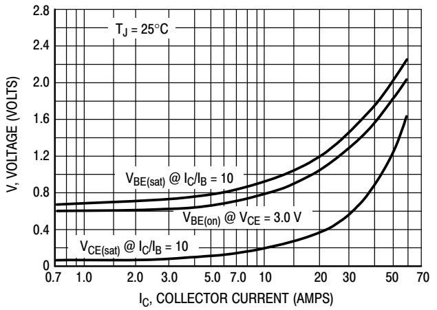
Figure 8. "On" Voltages
