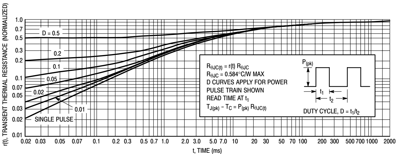
Figure 13. Thermal Response
