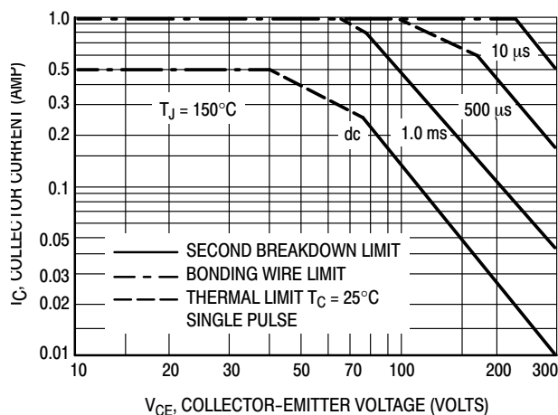
Figure 3. MJE340
