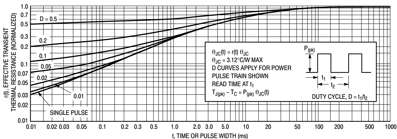
Figure 6. Thermal Response
