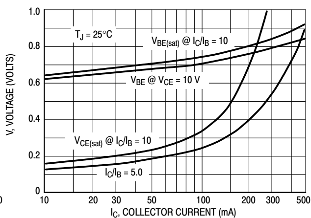
Figure 2. "On" Voltages
