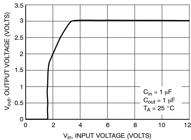
Figure 10. Output Voltage versus Input Voltage
