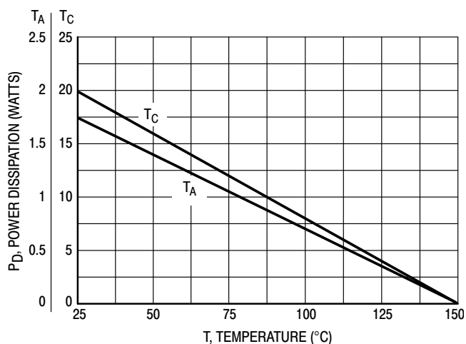
Figure 2. Power Derating
