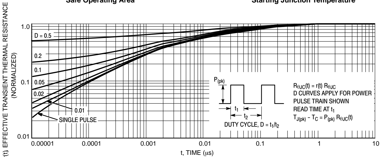
Figure 13. Thermal Response
