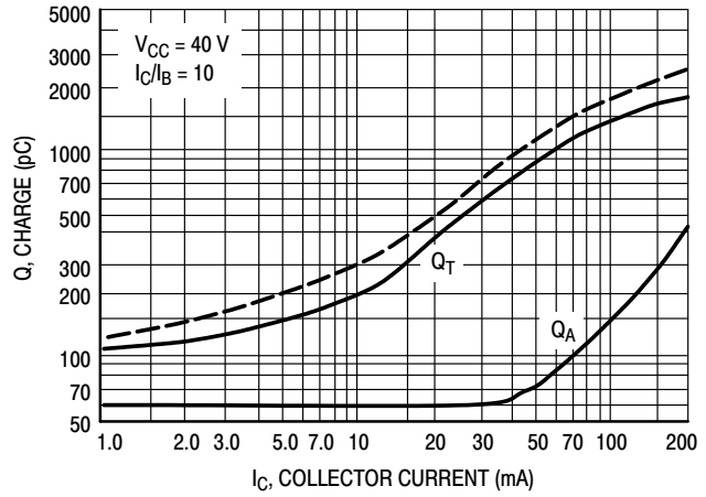
Figure 4. Charge Data
