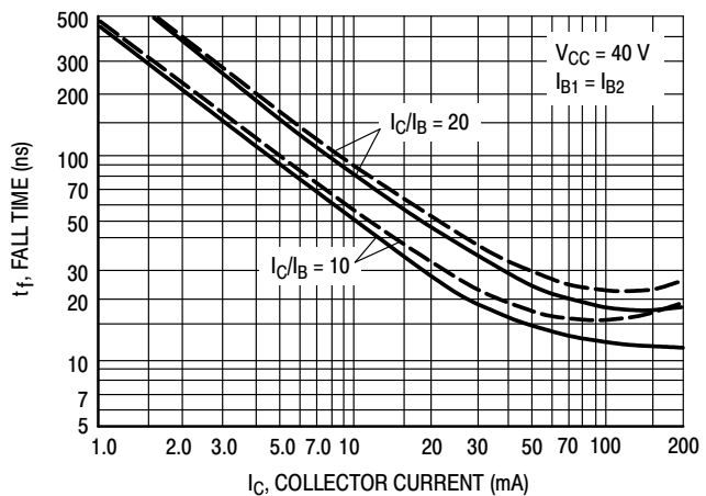
Figure 8. Fall Time
