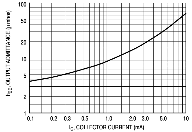
Figure 12. Output Admittance
