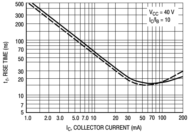
Figure 6. Rise Time
