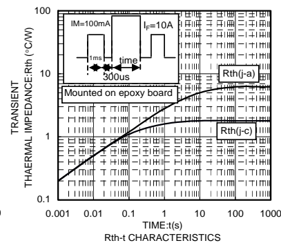
R_{th} \cdot t CHARACTERISTICS
