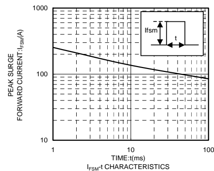
I_{FSM} \cdot t CHARACTERISTICS
