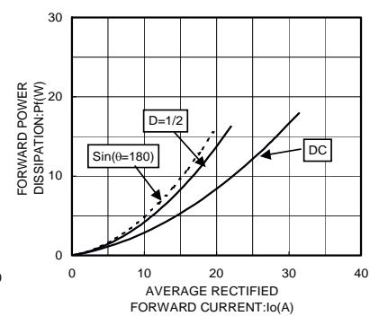
I_o \cdot P_f CHARACTERISTICS
