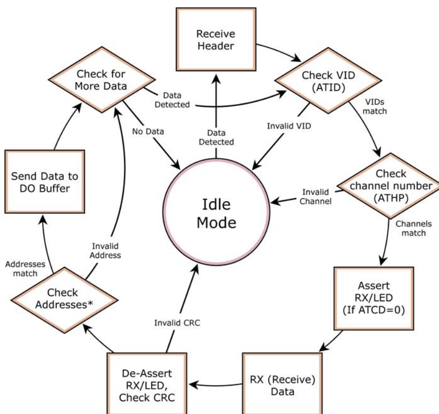
Figure 3-05. Receive Mode Data Flow
