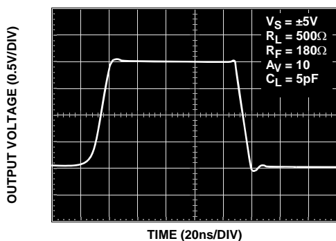
FIGURE 21. LARGE SIGNAL STEP RESPONSE
