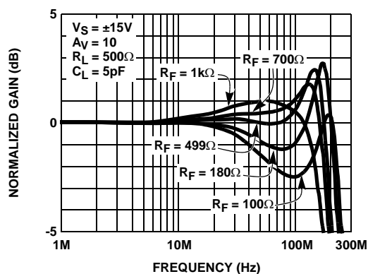
FIGURE 2. NON-INVERTING FREQUENCY RESPONSE FOR VARIOUS R_F
