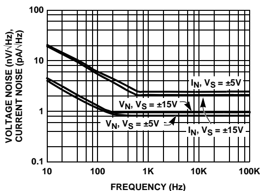
FIGURE 26. VOLTAGE AND CURRENT NOISE vs FREQUENCY
