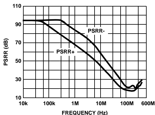
FIGURE 30. PSRR
