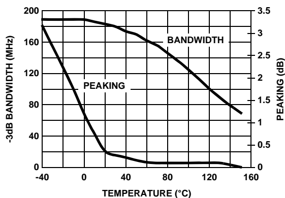
FIGURE 32. BANDWIDTH vs TEMPERATURE
