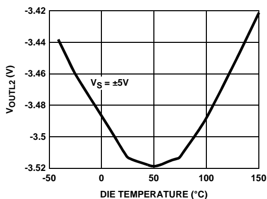
FIGURE 44. LOADED NEGATIVE OUTPUT SWING vs TEMPERATURE
