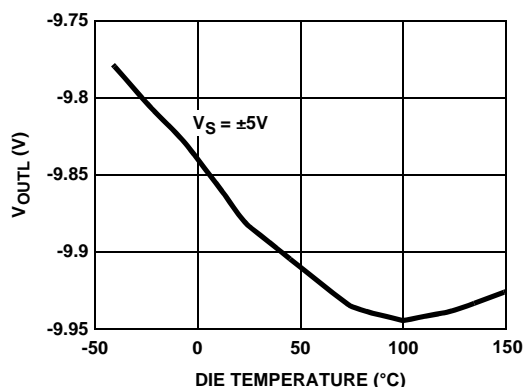
FIGURE 42. NEGATIVE OUTPUT SWING vs TEMPERATURE
