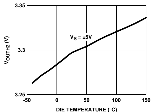
FIGURE 46. LOADED POSITIVE OUTPUT SWING vs TEMPERATURE
