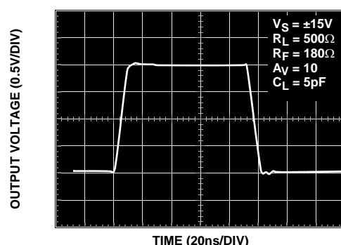
FIGURE 22. LARGE SIGNAL STEP RESPONSE
