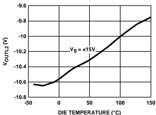
FIGURE 45. NEGATIVE OUTPUT SWING vs TEMPERATURE
