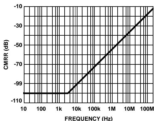
FIGURE 29. CMRR
