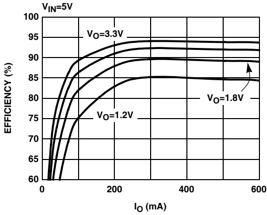
FIGURE 1. EFFICIENCY
