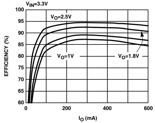
FIGURE 2. EFFICIENCY
