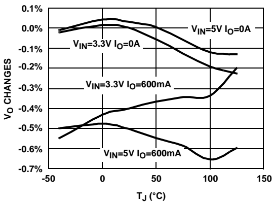
FIGURE 5. LOAD/LINE REGULATIONS vs JUNCTION TEMPERATURE
