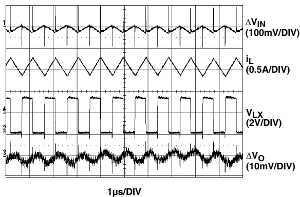
FIGURE 11. STEADY-STATE
