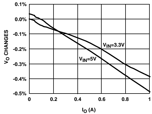
FIGURE 4. LOAD REGULATIONS
