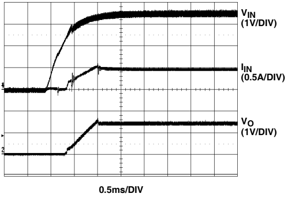
FIGURE 7. START-UP 1
