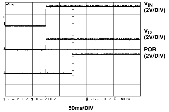
FIGURE 8. START-UP 2
