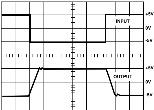
Vertical = 5V/Div., Horizontal = 5μs/Div. ( A_V = -1 )
