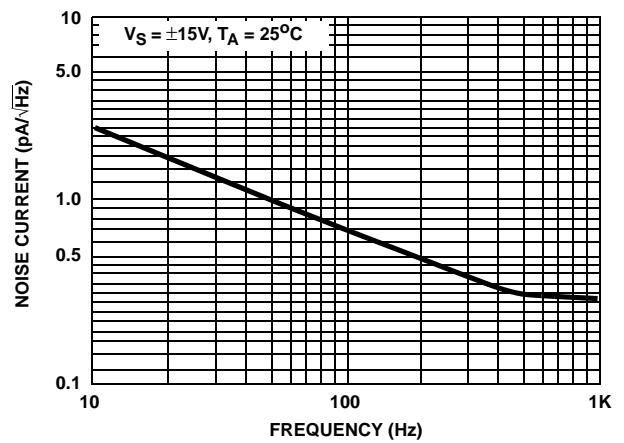
FIGURE 5. INPUT NOISE CURRENT DENSITY
