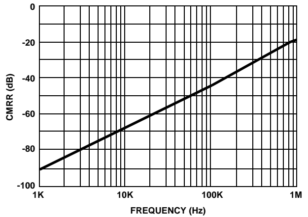
FIGURE 19. CMRR vs FREQUENCY
