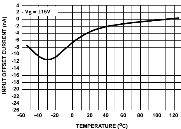
FIGURE 10. I_{IO} vs TEMPERATURE
