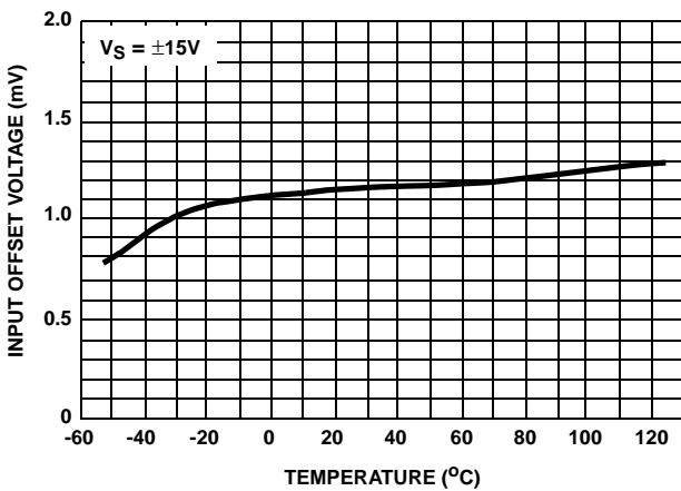
FIGURE 8. V_{IO} vs TEMPERATURE
