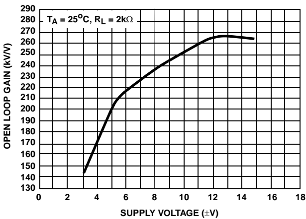
FIGURE 16. A_{VOL} vs V_S
