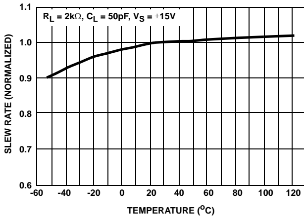
FIGURE 24. SLEW RATE vs TEMPERATURE
