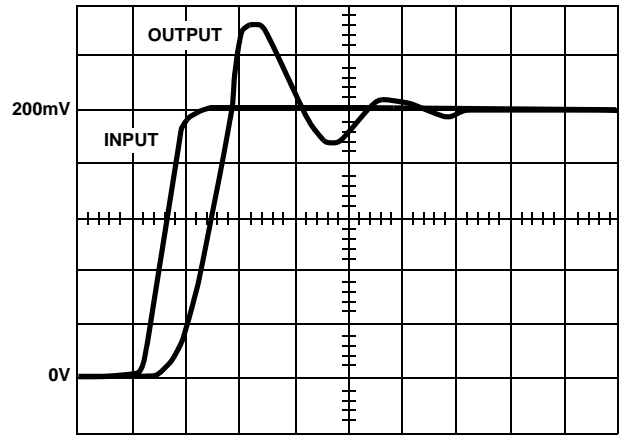
Vertical = 40mV/Div., Horizontal = 50ns/Div. ( A_V = +1 )
