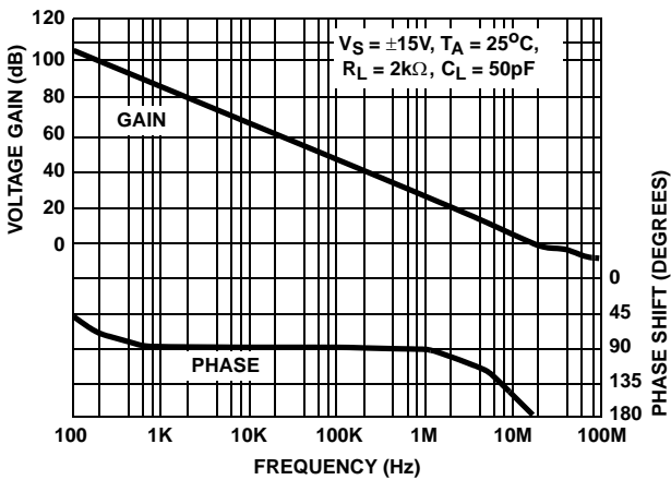
FIGURE 22. OPEN LOOP GAIN vs FREQUENCY
