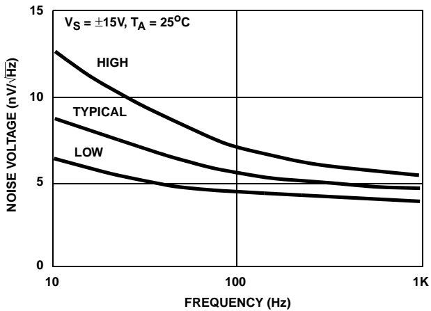
FIGURE 4. INPUT NOISE VOLTAGE DENSITY
