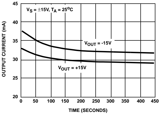
FIGURE 18. OUTPUT SHORT CIRCUIT CURRENT vs TIME
