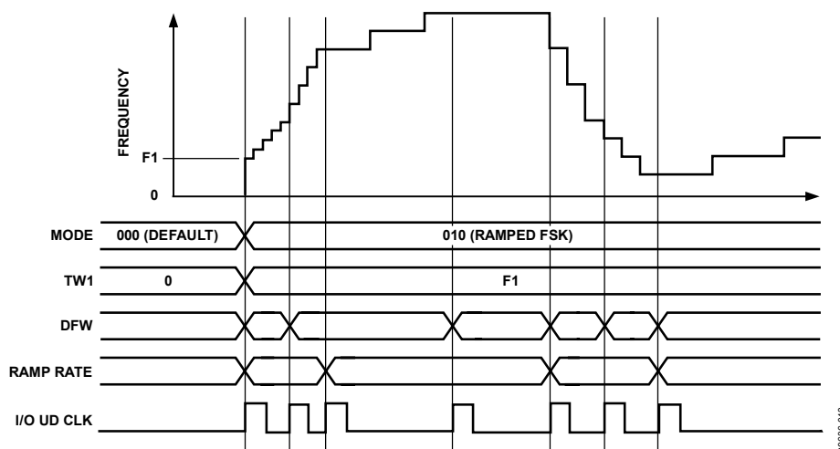
Figure 43. Example of a Nonlinear Chirp
