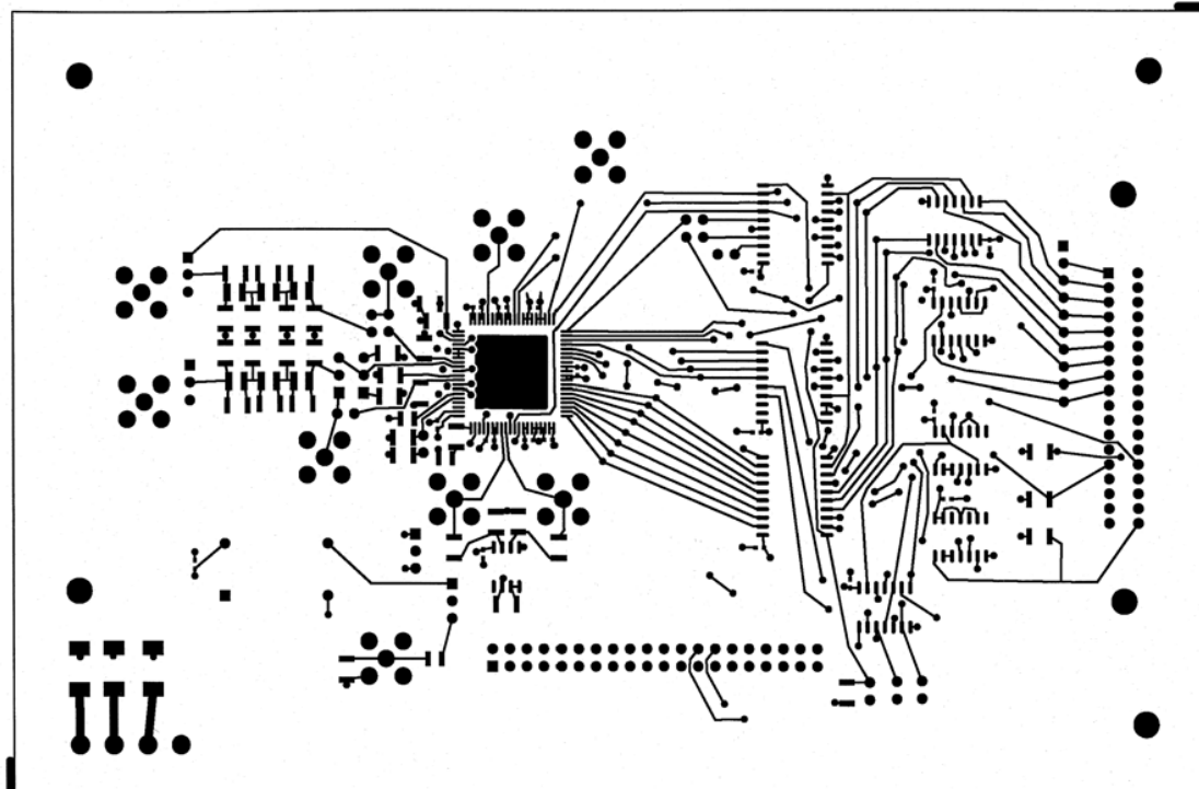
Figure 67. Top Routing Layer, Layer 1
