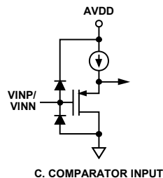
Figure 3. Equivalent Input and Output Circuits
