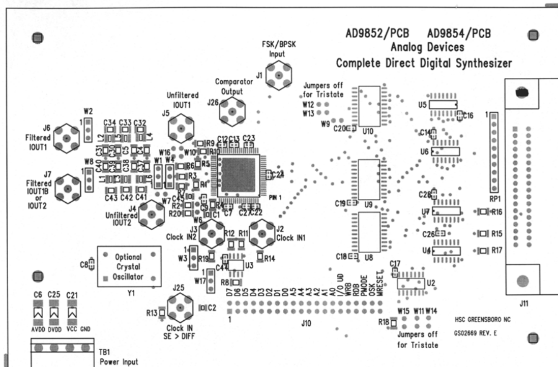
Figure 66. Assembly Drawing
