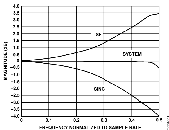
Figure 51. Inverse Sinc Filter Response
