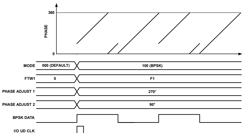
Figure 48. BPSK Mode
