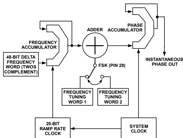
Figure 39. Block Diagram of Ramped FSK Function
