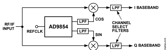
Figure 25. Quadrature Downconversion
