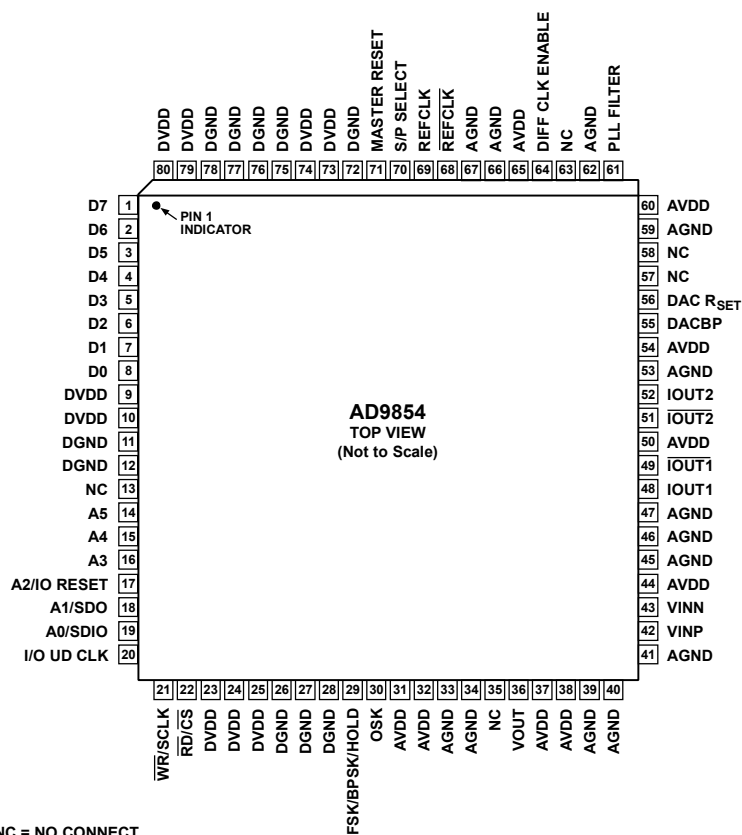
Figure 2. Pin Configuration
