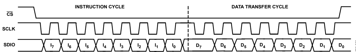
Figure 60. Serial Port Write Timing Clock Stall High
