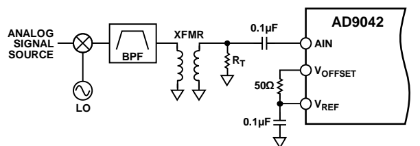
Figure 34. Transformer-Coupled Analog Input Signal
