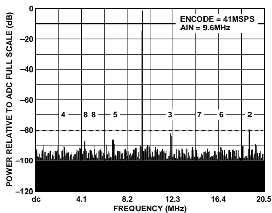
Figure 4. Single Tone at 9.6 MHz
