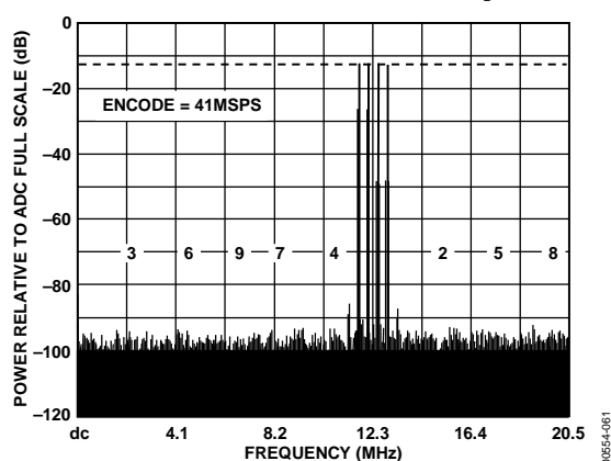
Figure 43. Multitone Performance
