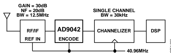
Figure 42. Receiver Analysis
