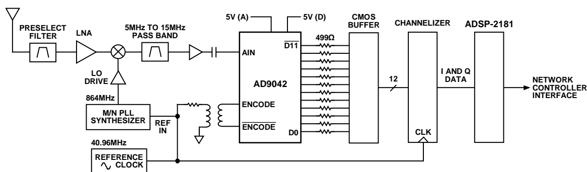
Figure 39. Simplified 5 MHz Wideband "A" Carrier Receiver
