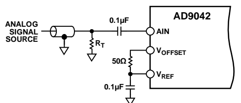
Figure 33. AC-Coupled Analog Input Signal
