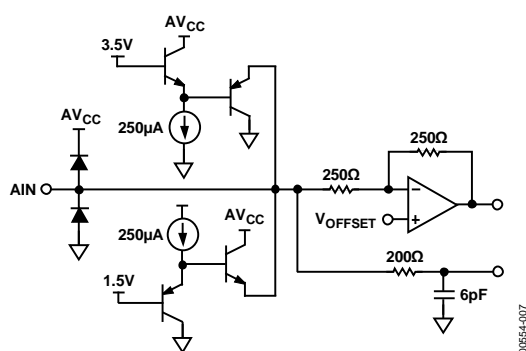
Figure 20. Analog Input Stage
