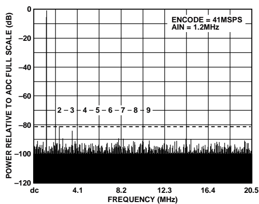
Figure 3. Single Tone at 1.2 MHz
