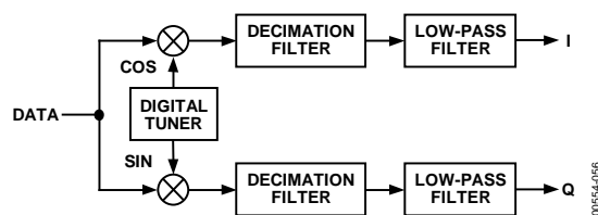
Figure 38. Digital Channelizer
