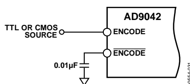
Figure 25. Single-Ended TTL/CMOS Encode
