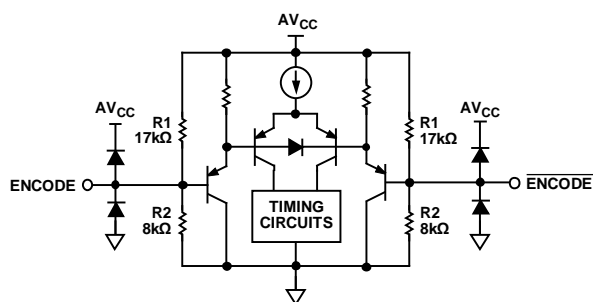
Figure 21. Encode Inputs
