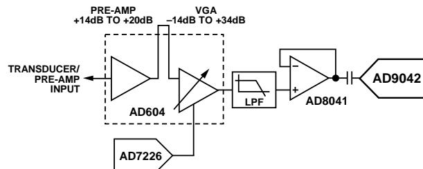
Figure 45. Using the AD9042 in Ultrasound Applications
