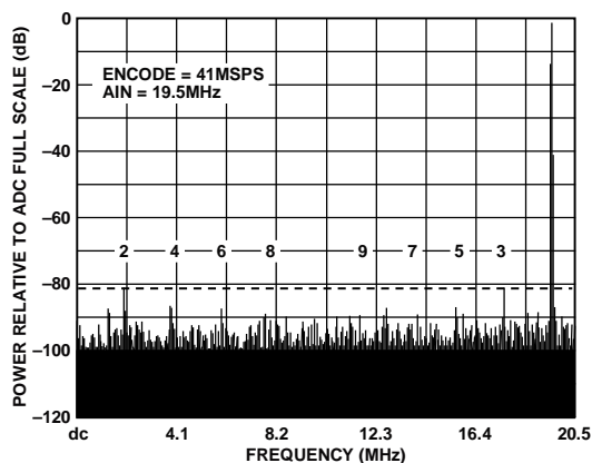
Figure 5. Single Tone at 19.5 MHz
