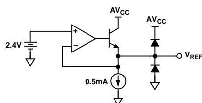
Figure 24. 2.4 V Reference
