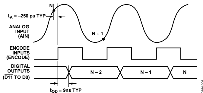
Figure 19. Timing Diagram
