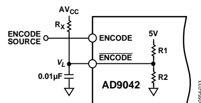
Figure 27. Raise Logic Threshold for Encode
