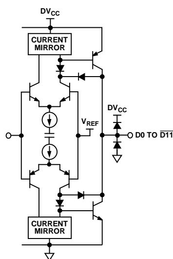
Figure 23. Digital Output Stage
