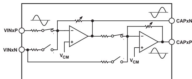
Figure 11. Single-Ended Analog Input
