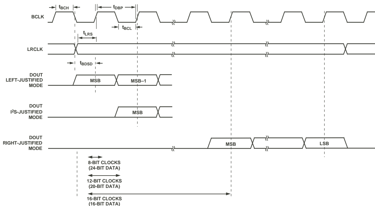
Figure 3. Slave Data Interface Timing
