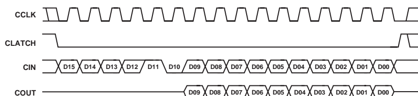
Figure 21. Reading from Register Using Control Port
