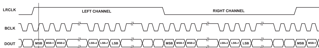
Figure 13. Left-Justified Mode
