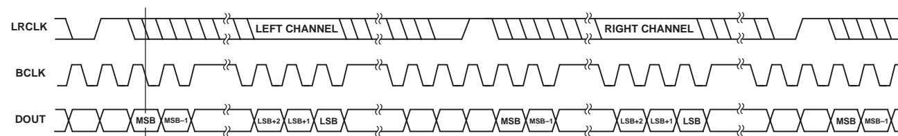
Figure 15. DSP Mode
