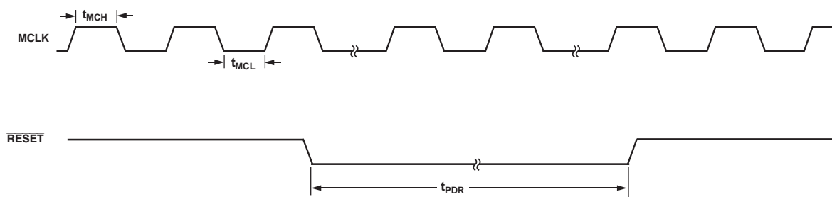
Figure 1. MCLK/ \overline{\text{RESET}} Timing
