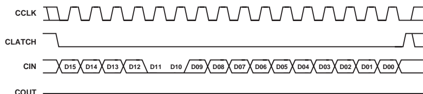
Figure 20. Writing to Register Using Control Port
