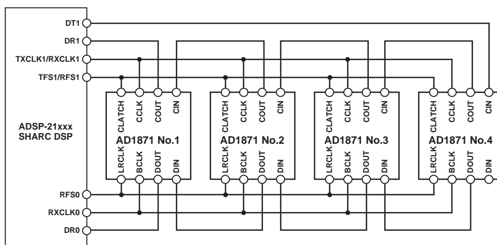
Figure 17. DSP Mode
