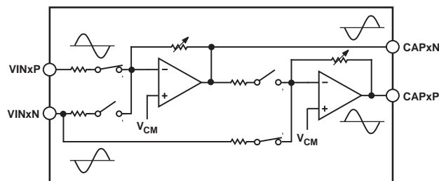
Figure 10. Differential Analog Input
