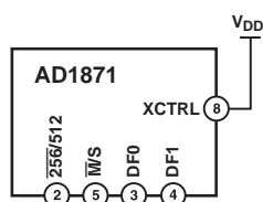
Figure 22. External Control Configuration
