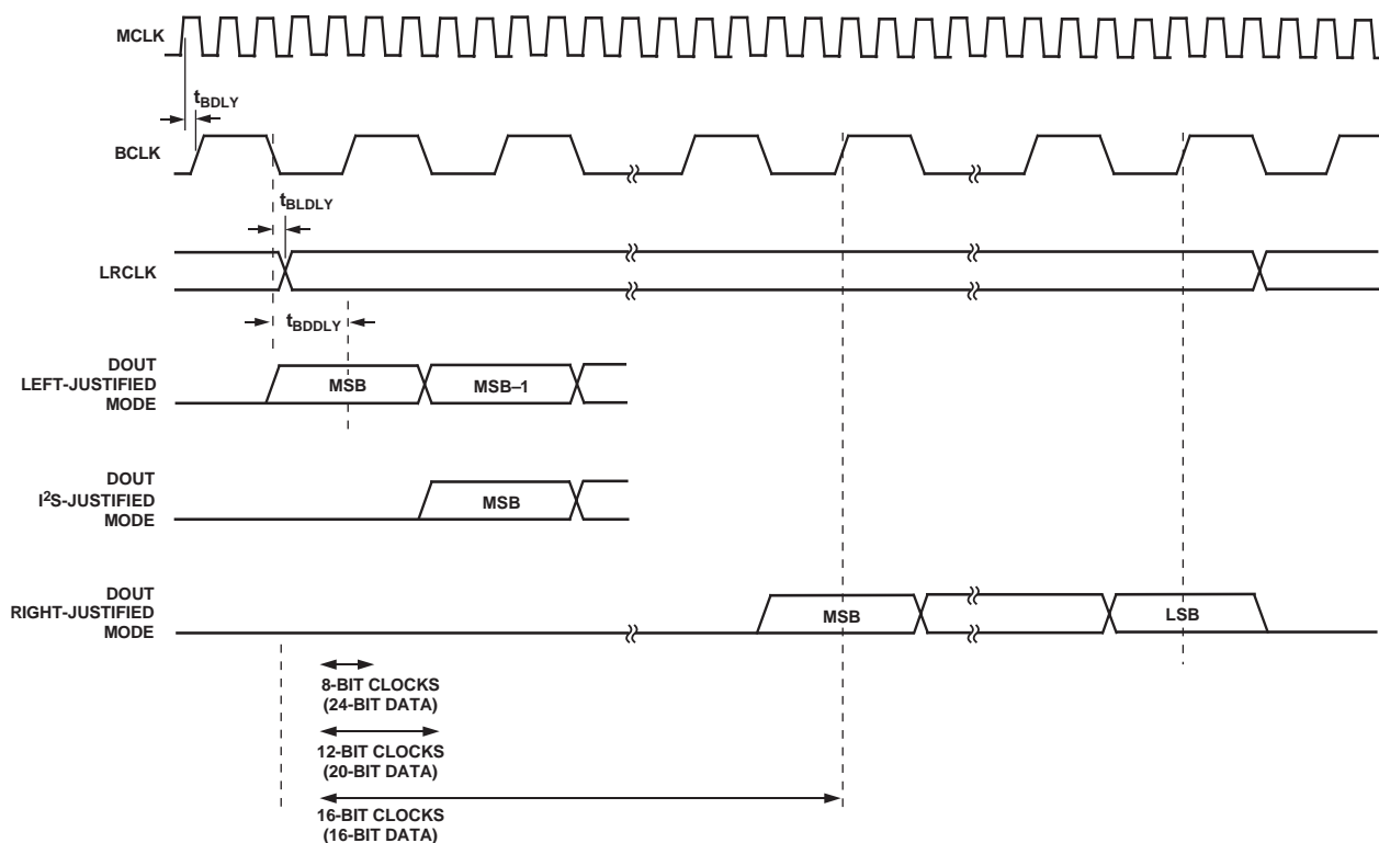
Figure 2. Master Data Interface Timing
