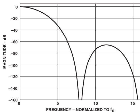
TPC 1. Sinc Filter Response (AMC = 0)
