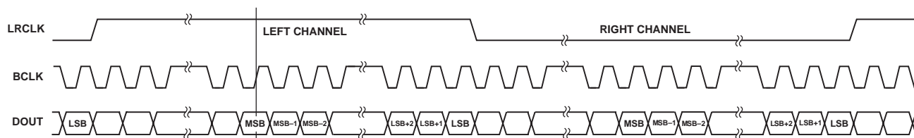
Figure 14. Right-Justified Mode
