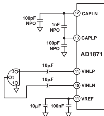
Figure 25. Differential Input via PGA Section
