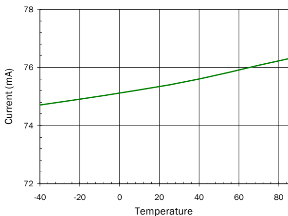
I b versus Temperature
