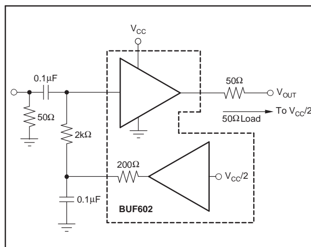
Figure 32. AC-Coupled, Single-Supply, Specification and Test Circuit
