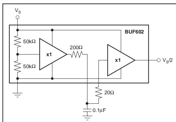
Figure 34. Self-Biased, Low Impedance Mid-Supply Voltage Reference
