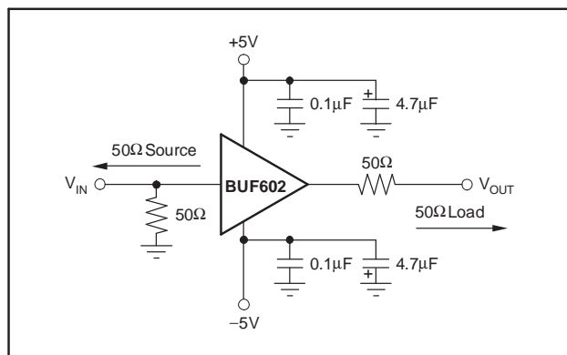
Figure 31. DC-Coupled, Bipolar Supply, Specification and Test Circuit
