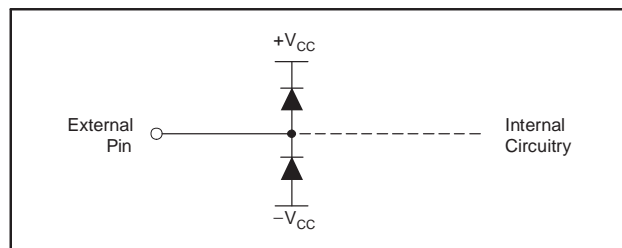
Figure 36. Internal ESD Protection
