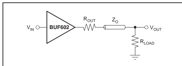
Figure 33. Typical Line Driver Circuit
