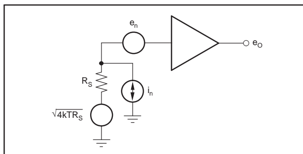
Figure 35. Buffer Noise Analysis Model
