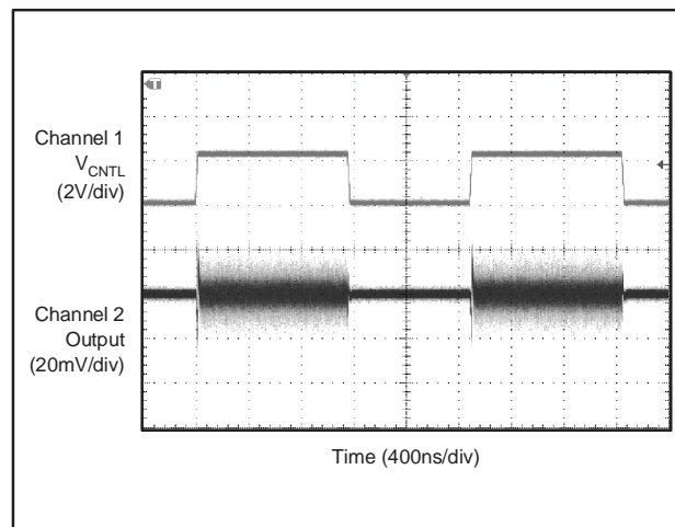
Figure 64. Response to Step Change of V_{CNTL}
