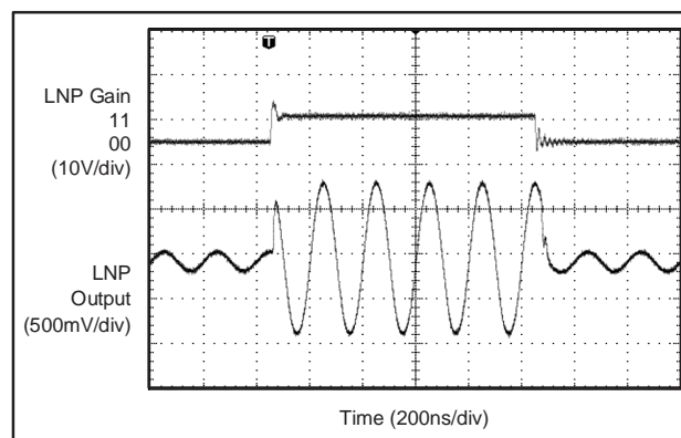
Figure 57. LNP Gain Change Response
