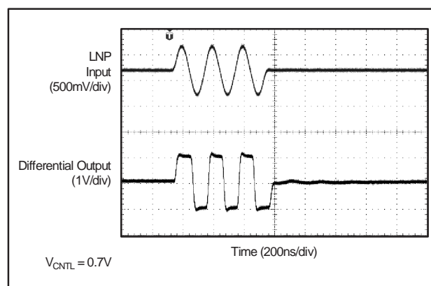
Figure 70. Extreme Overload (2V PP Input)
