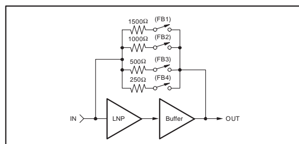
Figure 59. Feedback Resistor Network
