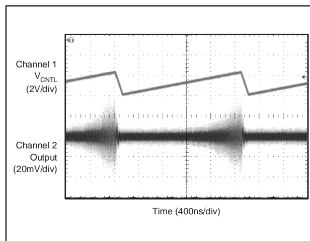
Figure 65. Response to Ramp Change of V_{CNTL}
