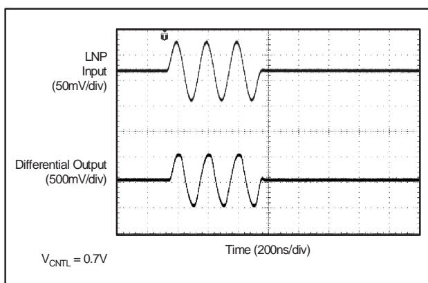
Figure 68. Approaching Overload (120mV PP Input)
