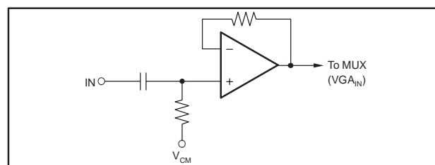
Figure 58. Recommended Circuit for Coupling an External Signal into the MUX
