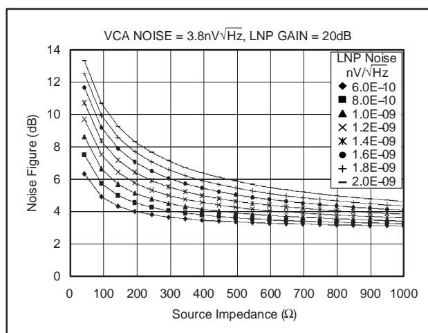
Figure 62. Noise Figure for Conventional Termination
