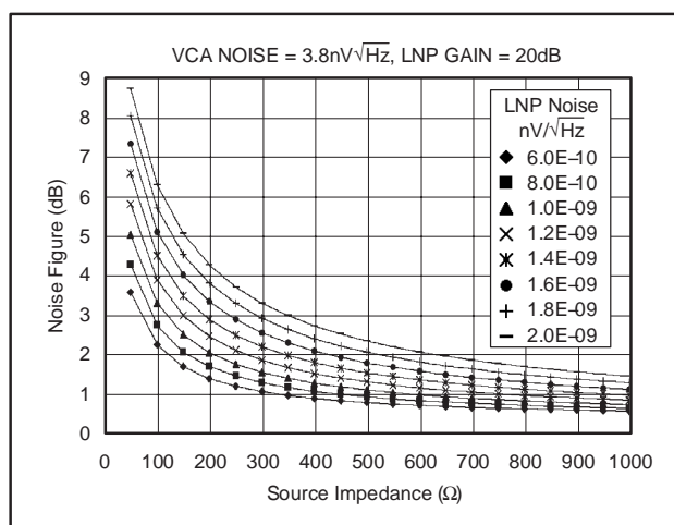
Figure 61. Noise Figure for Active Termination
