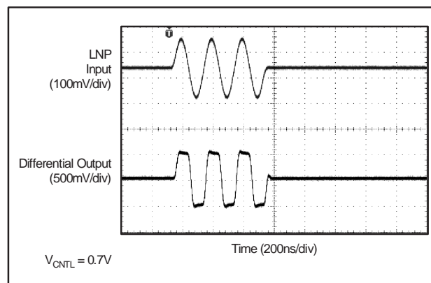
Figure 69. Overload (240mV PP Input)
