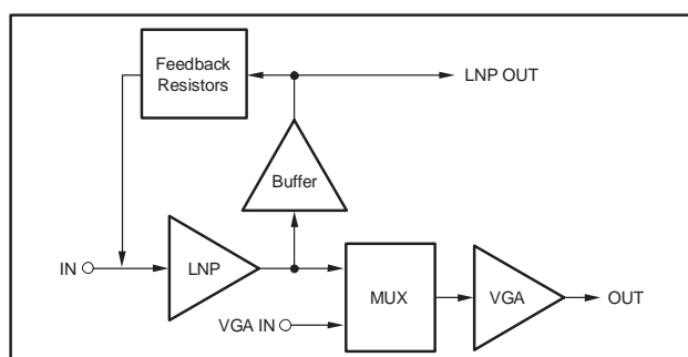
Figure 56. Block Diagram of LNP/VGA Interface
