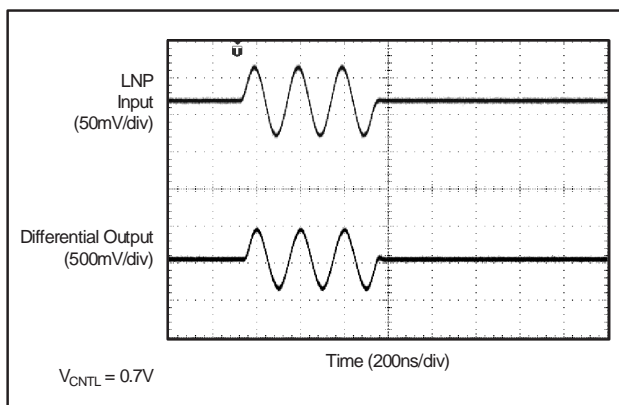
Figure 67. Before Overload (100mV PP Input)
