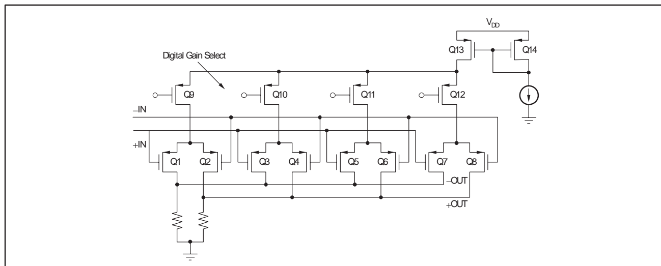
Figure 55. Programmable LNP
