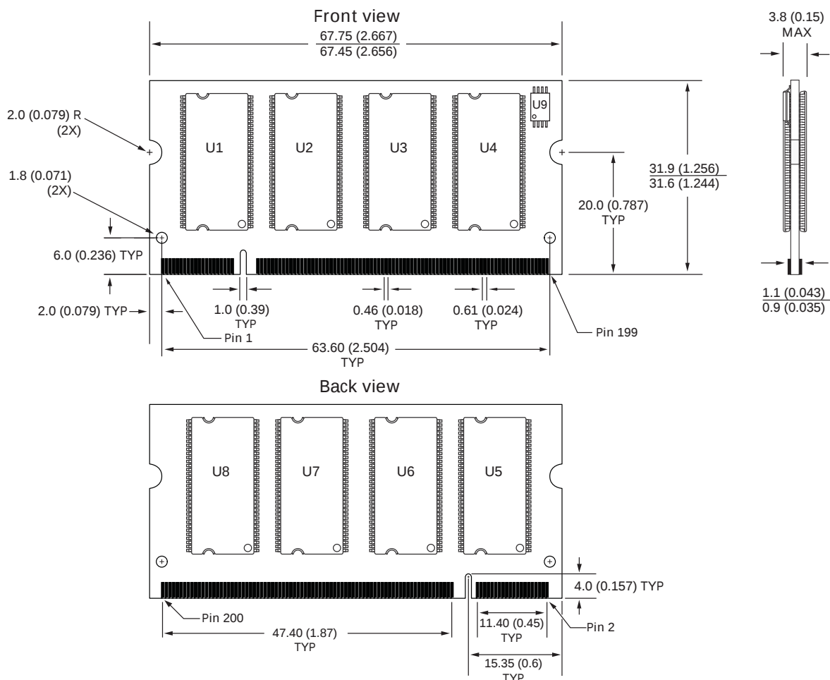
Figure 3: 200-Pin DDR SODIMM
