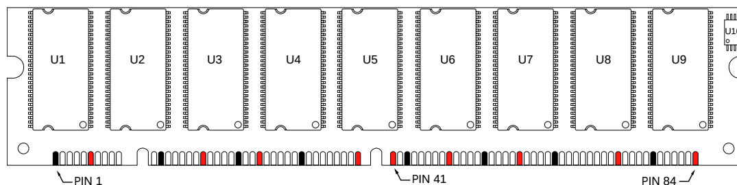
Figure 2: 168-Pin DIMM Pin Locations
