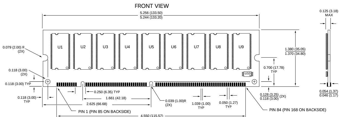
Figure 11: 168-Pin DIMM Dimensions – Single Rank
