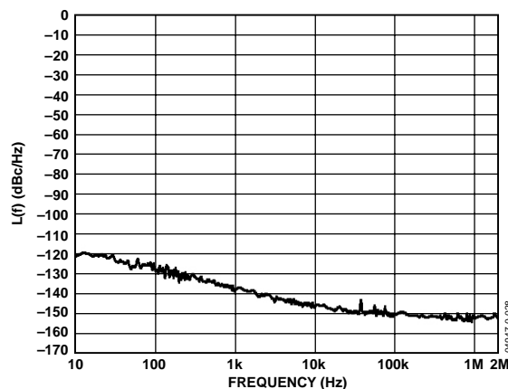
Figure 21. RF Divider and CML Driver Residual Phase Noise (157.6 MHz In, 19.7 MHz Out)
