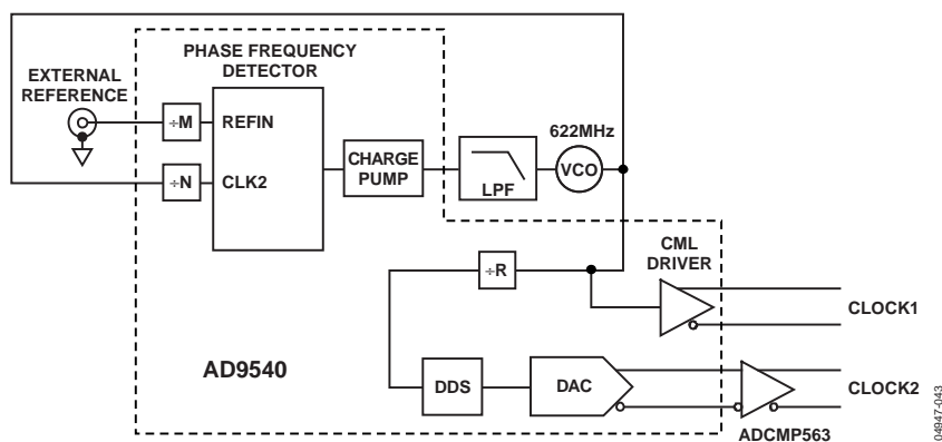
Figure 33. Optical Networking Clock
