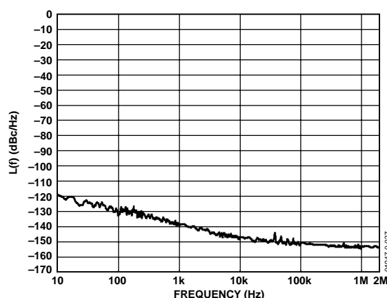
Figure 20. RF Divider and CML Driver Residual Phase Noise (81.92 MHz In, 10.24 MHz Out)
