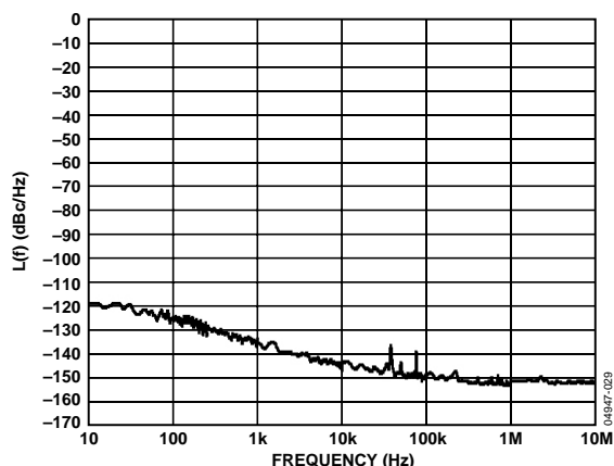
Figure 22. RF Divider and CML Driver Residual Phase Noise (410.4 MHz In, 51.3 MHz Out)
