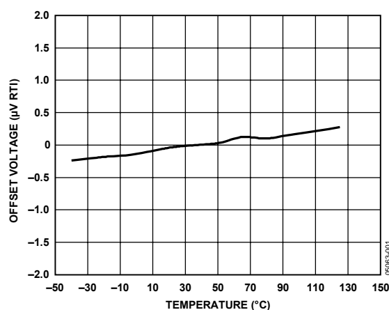
Figure 2. Relative Offset Voltage vs. Temperature
