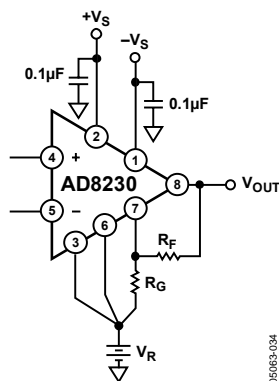
Figure 34. Level-Shifting the Output
