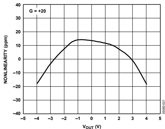
Figure 21. Gain Nonlinearity, G = 20
