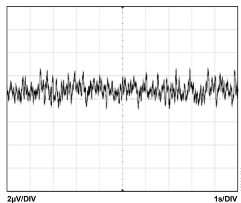
Figure 26. 0.1 Hz to 10 Hz RTI Voltage Noise, G = 100
