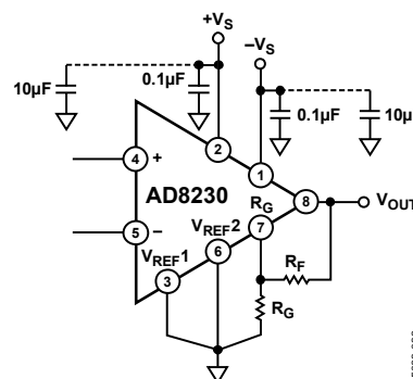
Figure 32. Gain Setting
