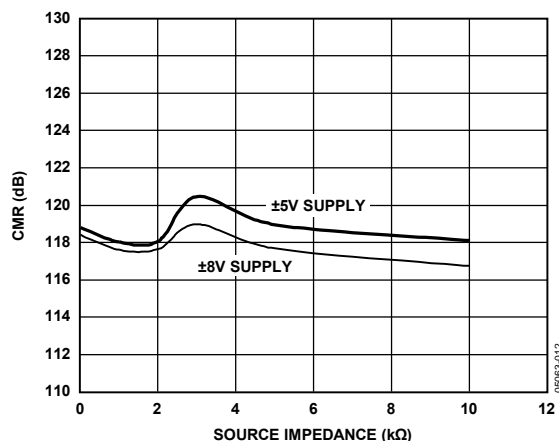
Figure 12. Common-Mode Rejection (CMR) vs. Source Impedance, 1.1 μF Across Input Pins
