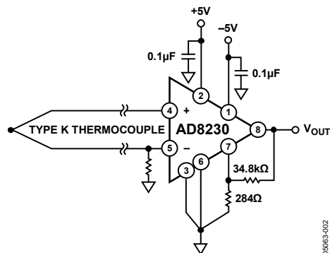
Figure 3. Thermocouple Measurement
