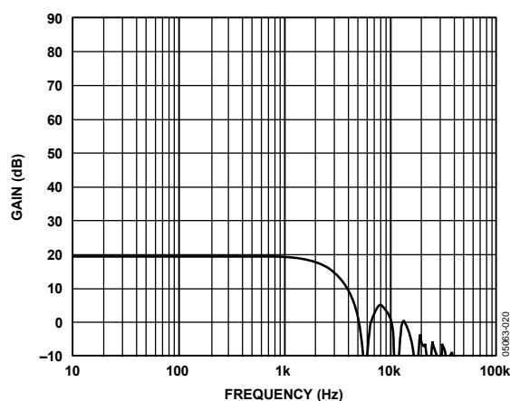
Figure 20. Gain vs. Frequency, G = 10
