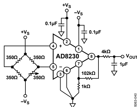
Figure 40. Bridge Measurement with Filtered Output
