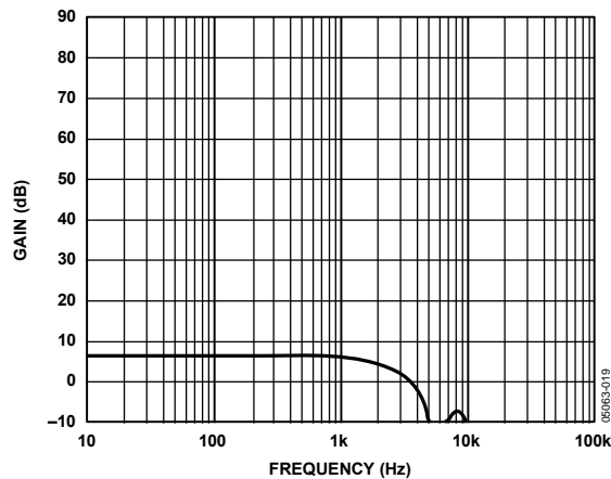
Figure 19. Gain vs. Frequency, G = 2
