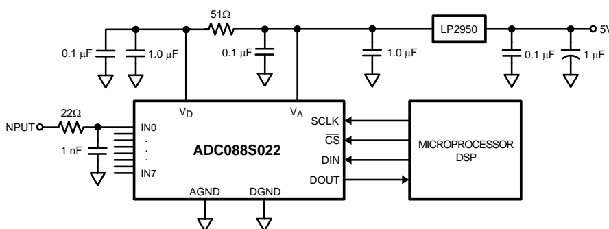
Figure 38. Typical Application Circuit
