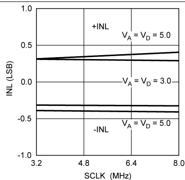
Figure 21. INL vs SCLK
