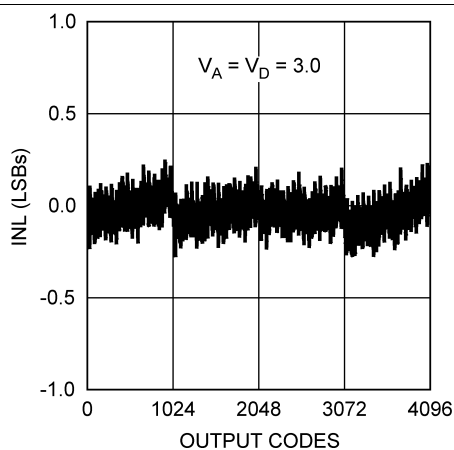
Figure 6. INL
