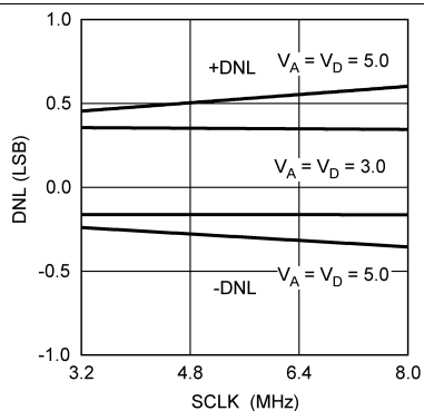
Figure 20. DNL vs SCLK
