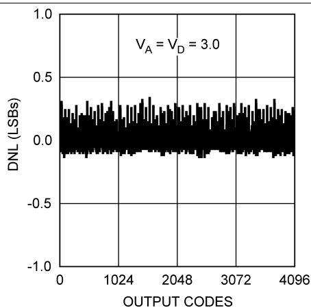
Figure 4. DNL
