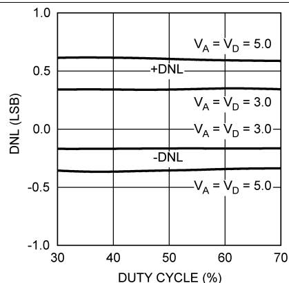
Figure 15. DNL vs SCLK Duty Cycle
