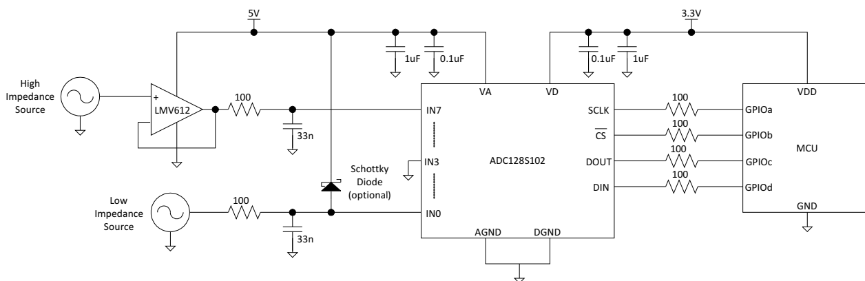
Figure 38. Typical Application Circuit
