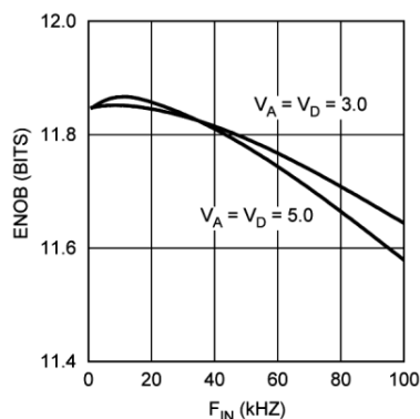
Figure 39. Typical Performance
