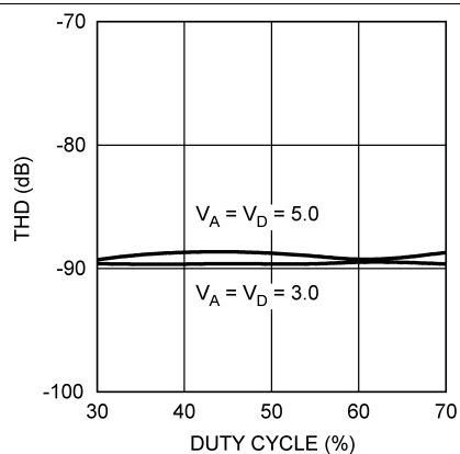
Figure 18. THD vs SCLK Duty Cycle
