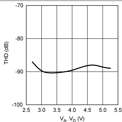
Figure 11. THD vs Supply
