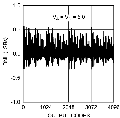
Figure 5. DNL
