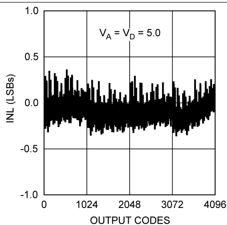
Figure 7. INL
