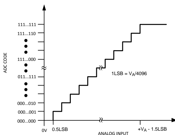
Figure 36. Ideal Transfer Characteristic
