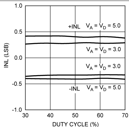
Figure 16. INL vs SCLK Duty Cycle
