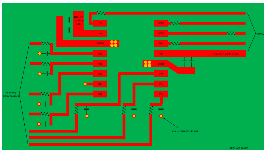
Figure 40. Layout Schematic
