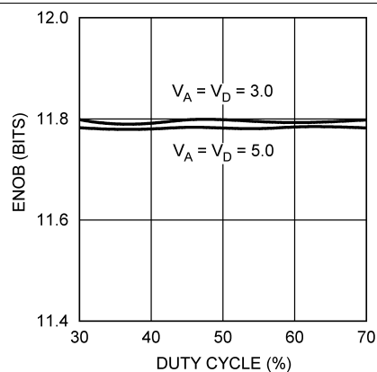
Figure 19. ENOB vs SCLK Duty Cycle
