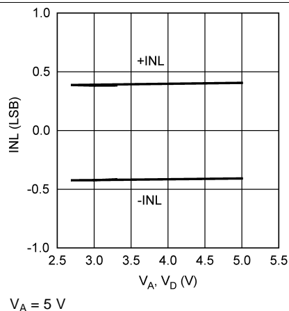
Figure 14. INL vs V_D
