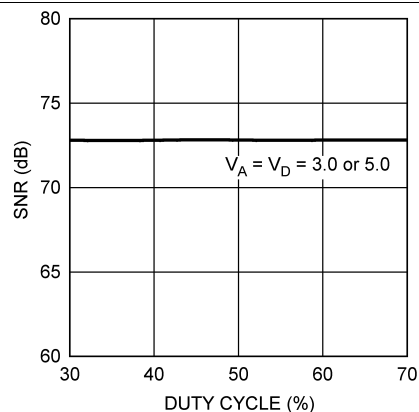
Figure 17. SNR vs SCLK Duty Cycle
