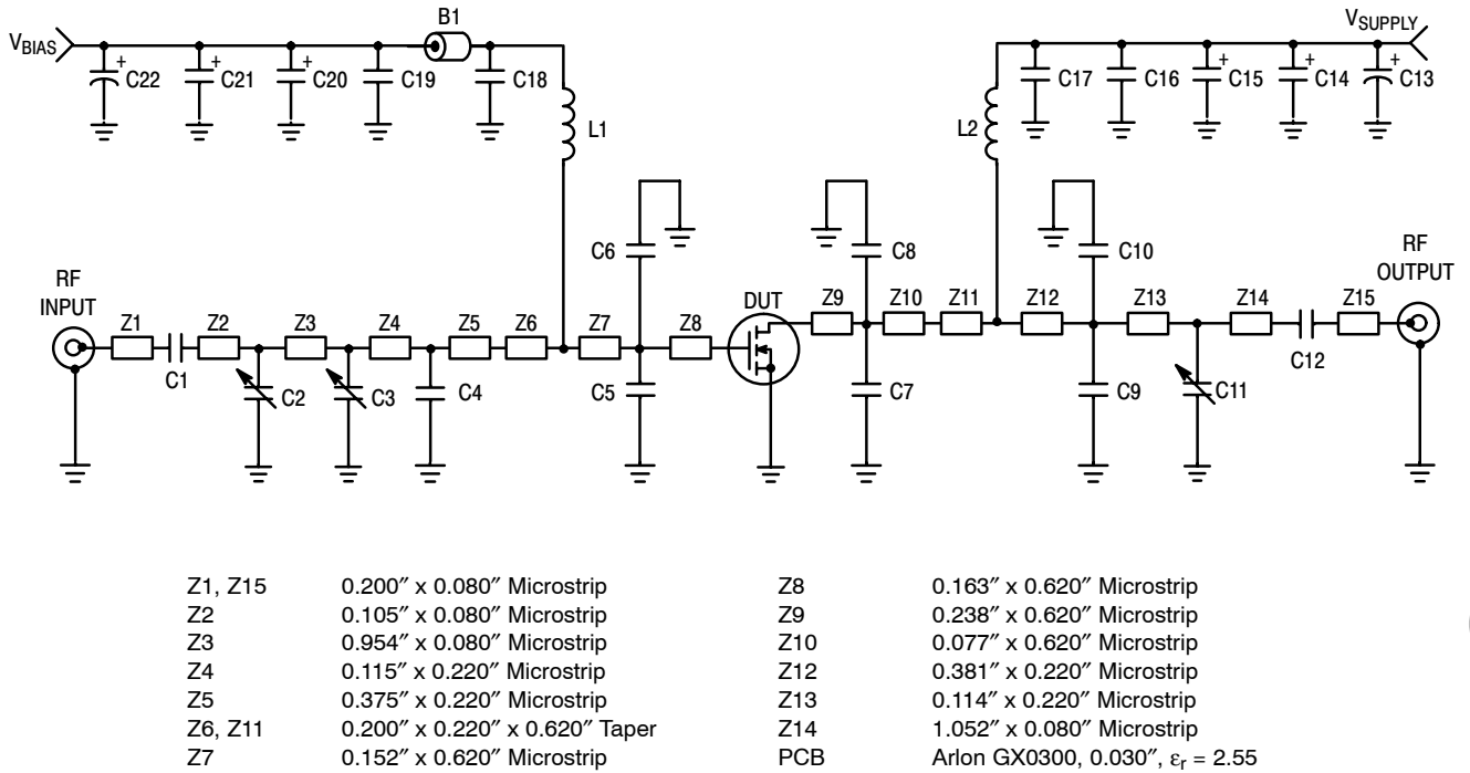
Figure 1. MRF5S9100MR1(MBR1) Test Circuit Schematic
