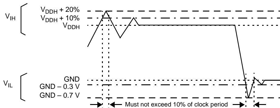
Figure 2-1. Overshoot/Undershoot Voltage for V_{IH} and V_{IL}
