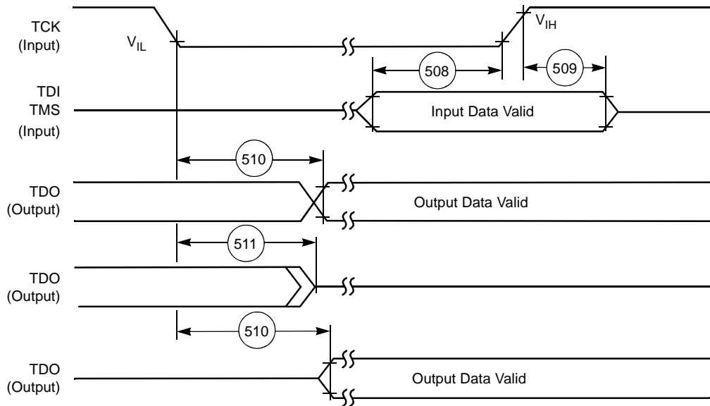
Figure 2-25. Test Access Port Timing Diagram
