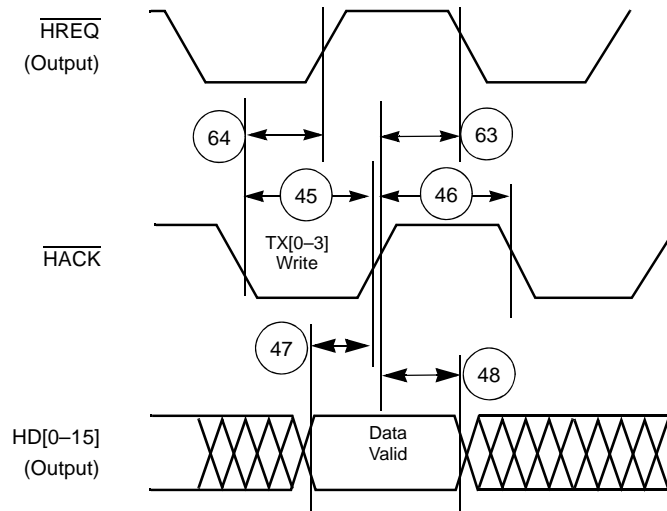
Figure 2-17. Host DMA Write Timing Diagram, HPCR[OAD] = 0
