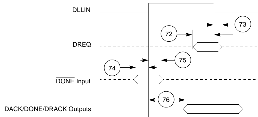
Figure 2-11. DMA Signals
