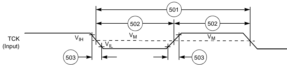
Figure 2-24. Test Clock Input Timing Diagram
