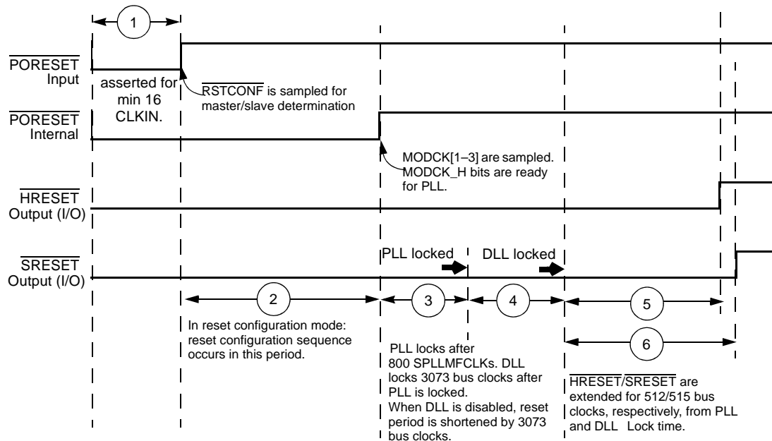
Figure 2-8. Hardware Reset Configuration Timing
