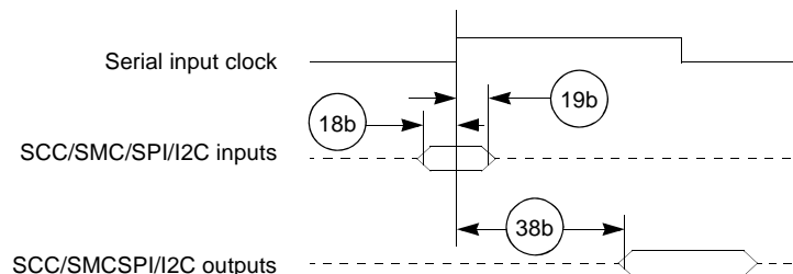
Figure 2-21. SCC/SMC/SPI/I 2 C External Clock Diagram
