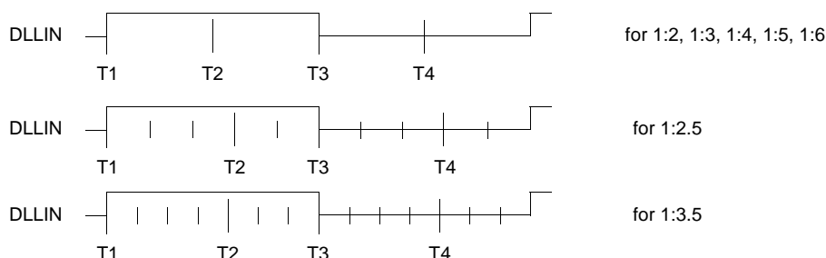
Figure 2-9. Internal Tick Spacing for Memory Controller Signals
