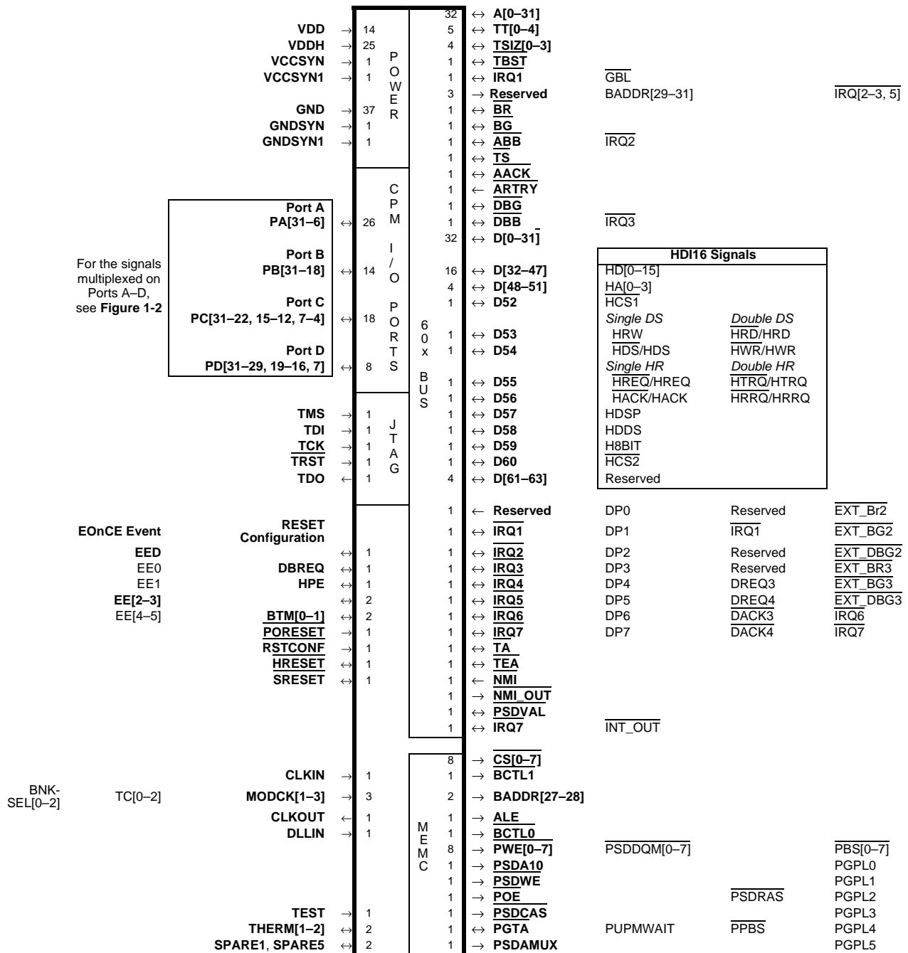
Figure 1-1. MSC8101 External Signals
