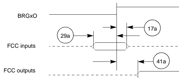
Figure 2-18. FCC Internal Clock Diagram
