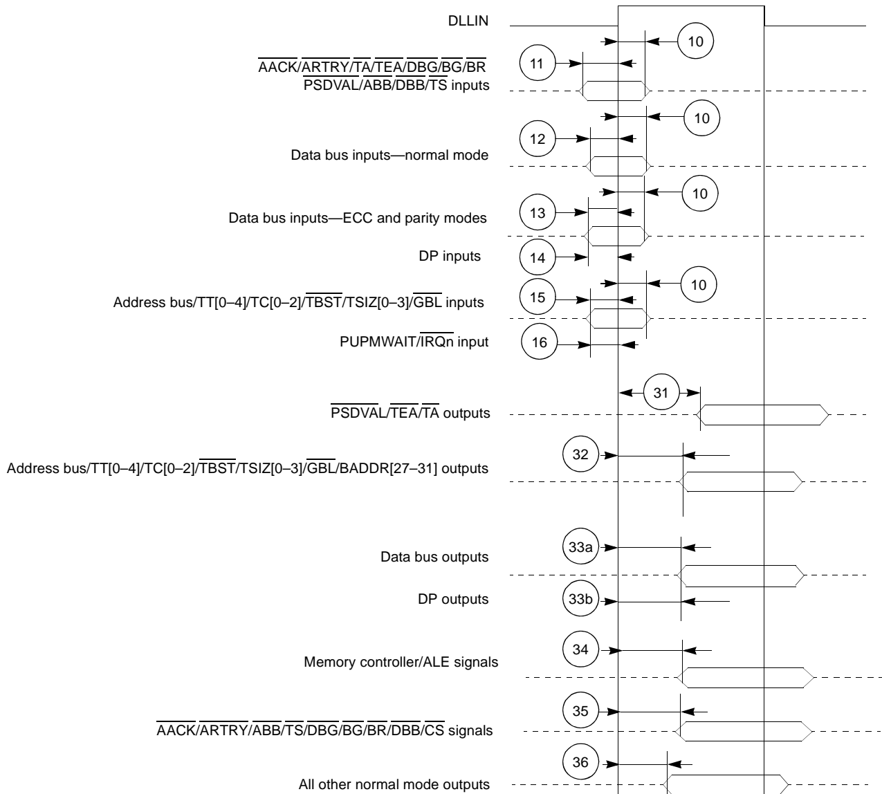
Figure 2-10. Bus Signal Timing
