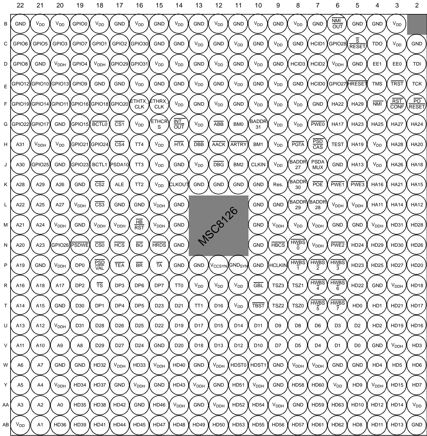
Bottom View
