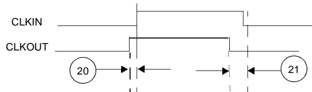
Figure 12. CLKOUT and CLKIN Signals.
