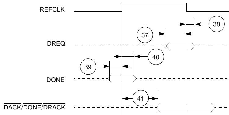
Figure 13. DMA Signals
