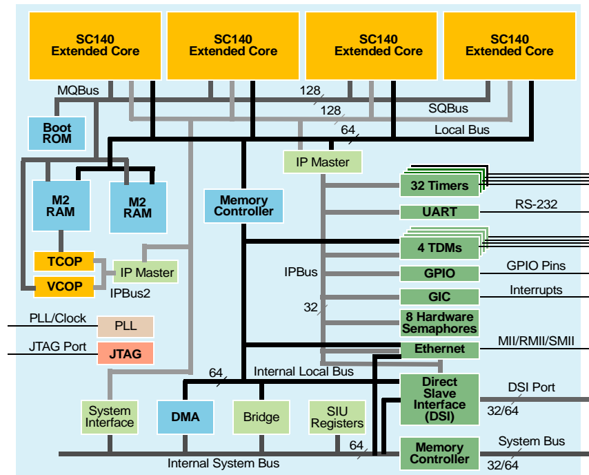
Figure 1. MSC8126 Block Diagram
