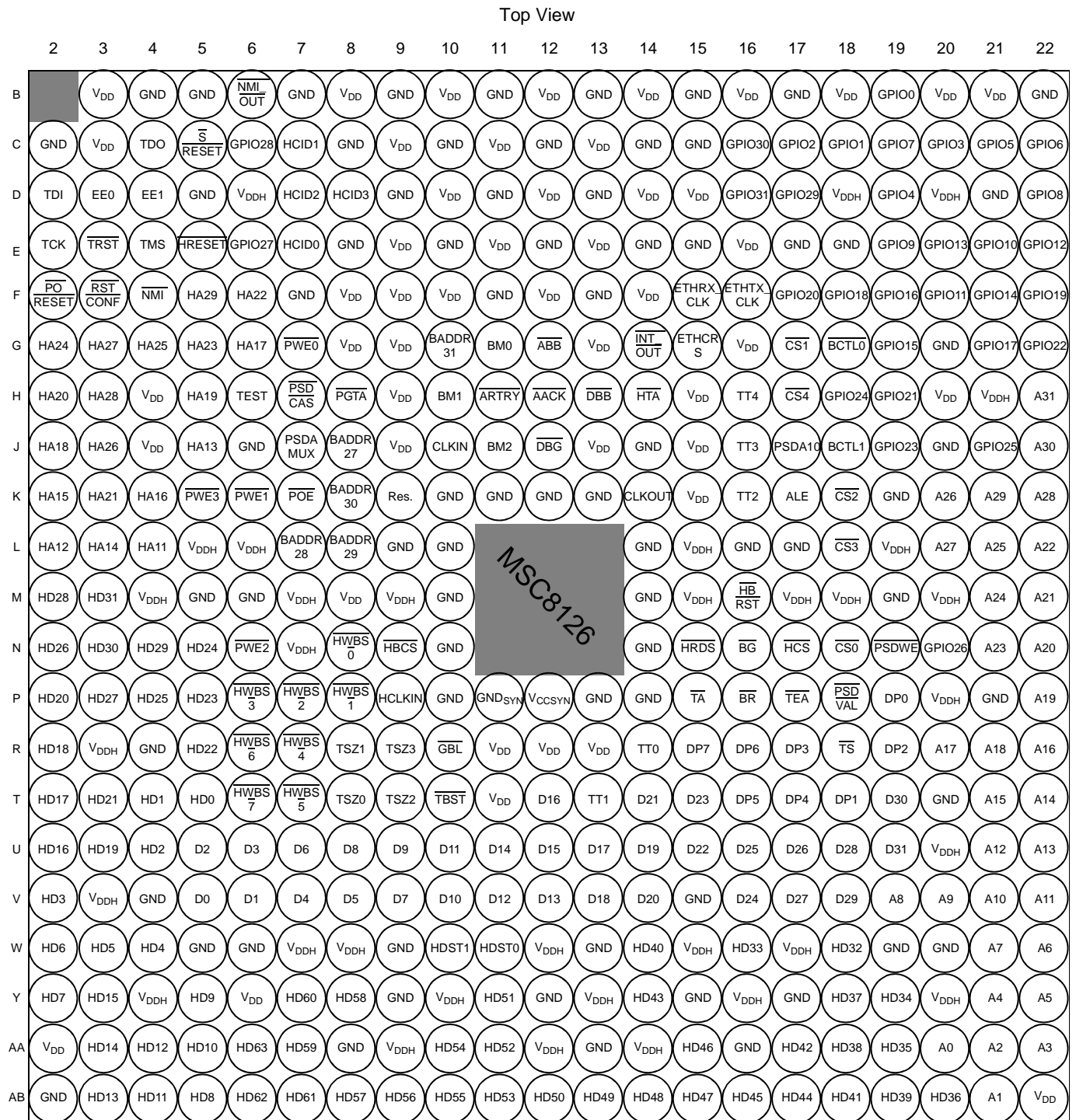
Figure 3. MSC8126 Package, Top View
