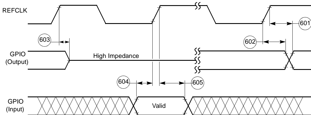
Figure 27. GPIO Timing
