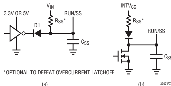
Figure 7. RUN/SS Pin Interfacing
