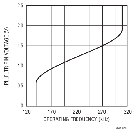
Figure 5. PLLFLTR Pin Voltage vs Frequency
