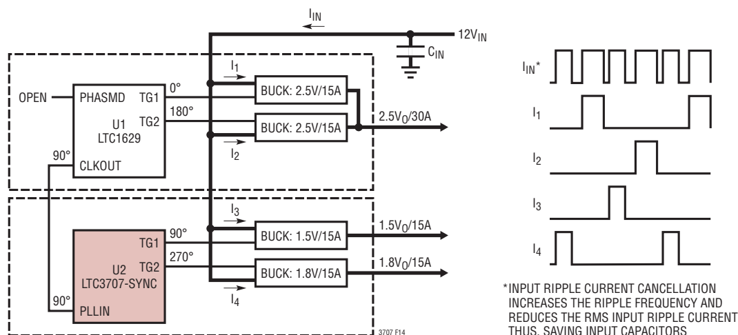
Figure 14. Multioutput Multiphase Application
