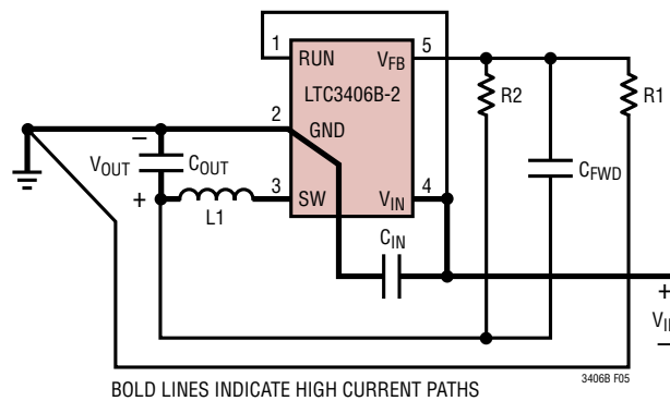
Figure 5. LTC3406B-2 Layout Diagram
