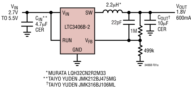
Figure 1a. High Efficiency Step-Down Converter
