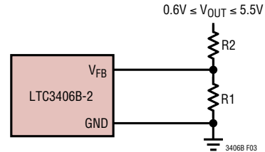
Figure 3. Setting the LTC3406B-2 Output Voltage
