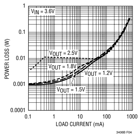
Figure 4. Power Lost vs Load Current
