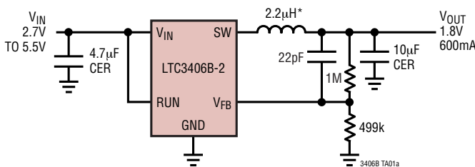
High Efficiency Step-Down Converter
