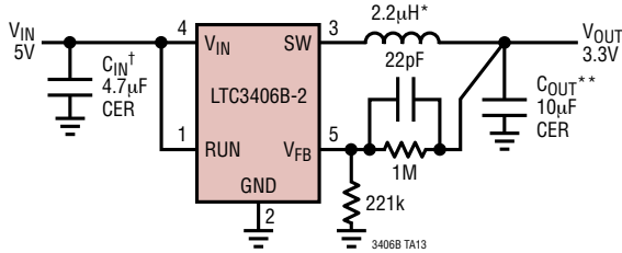
5V Input to 3.3V/0.6A Regulator
