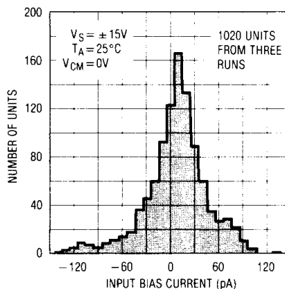
Typical Distribution of Input Bias Current
