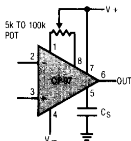
Optional Offset Nulling and Over-Compensation Circuits
