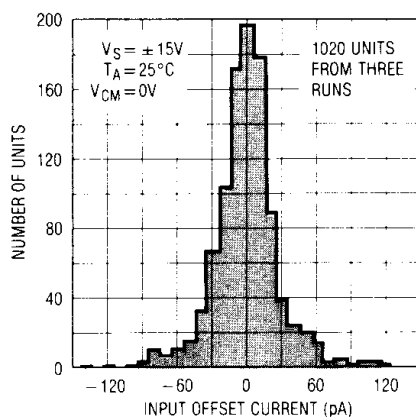
Typical Distribution of Input Offset Current
