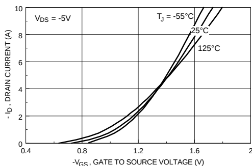
Figure 15. Transfer Characteristics.
