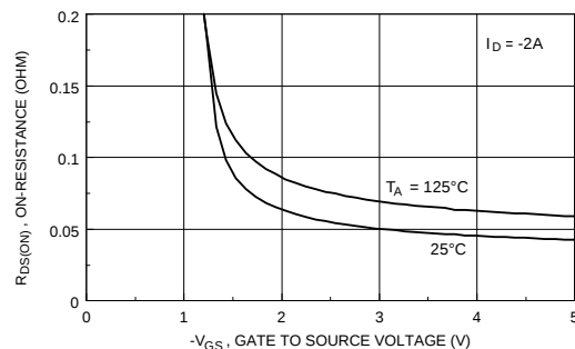
Figure 14. On-Resistance Variation with Gate-to-Source Voltage.
