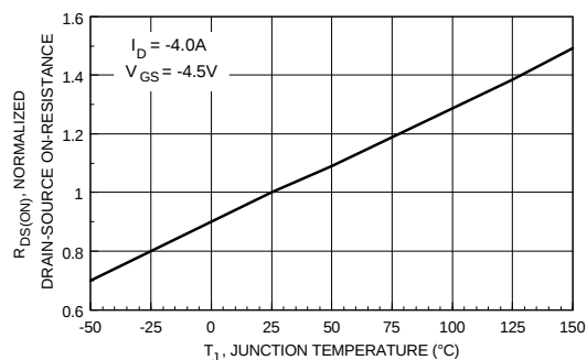
Figure 13. On-Resistance Variation with Temperature.
