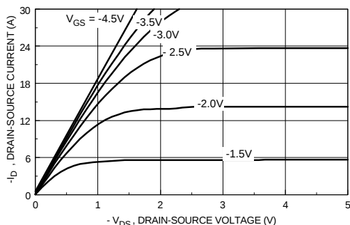
Figure 11. On-Region Characteristics.
