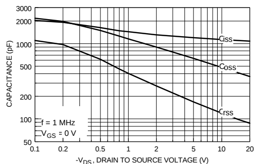
Figure 18. Capacitance Characteristics.
