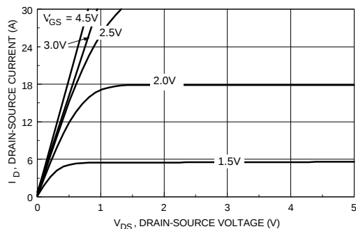
Figure 1. On-Region Characteristics.
