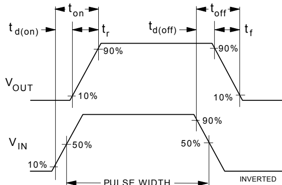
Figure 12. Switching Waveforms.
