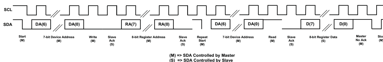
Figure 19. I 2 C Read
