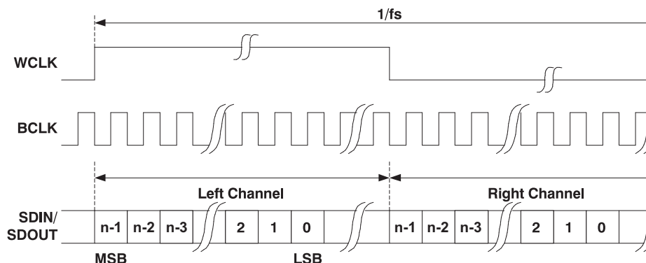
Figure 23. Left Justified Serial Data Bus Mode Operation
