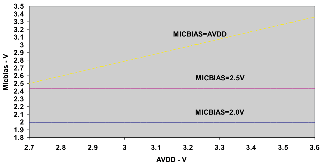
Figure 12. MICBIAS Output Voltage vs AVDD
