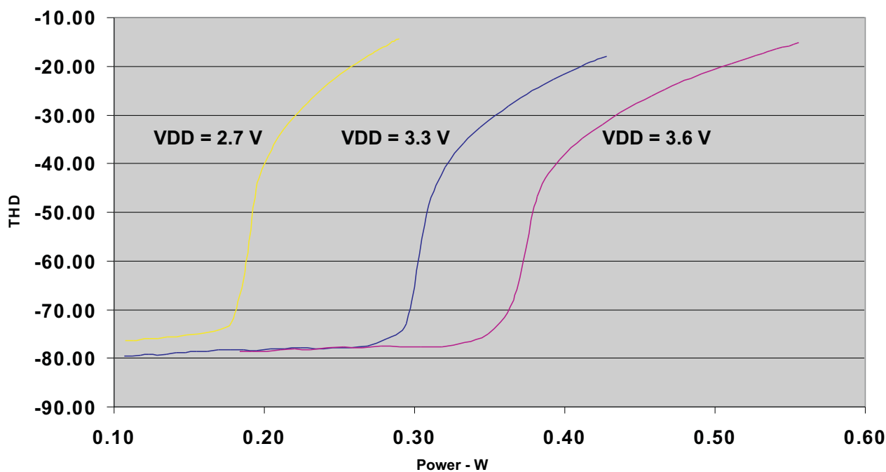
Figure 9. Speaker Power vs THD, 8 \Omega Load
