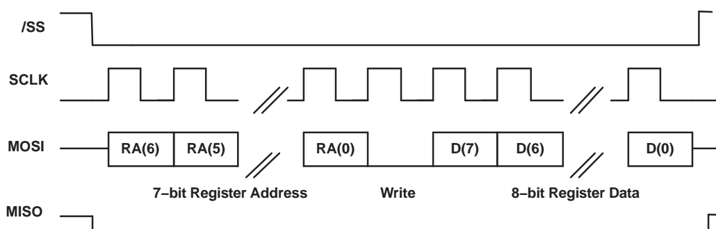
Figure 15. SPI Write
