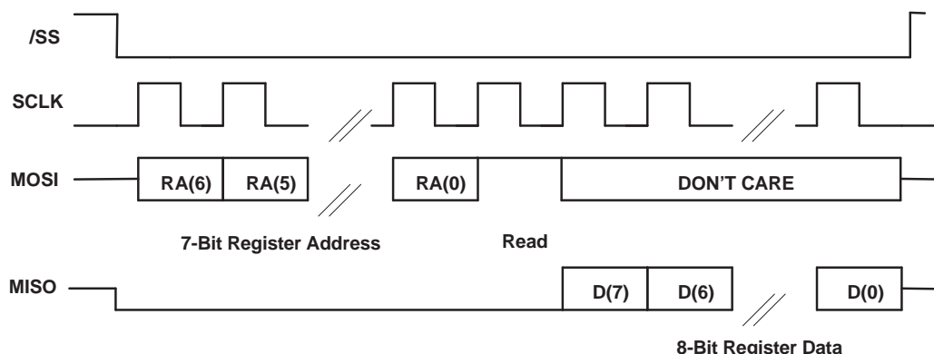
Figure 16. SPI Read
