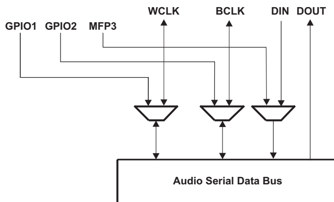
Figure 20. Alternate Audio Bus Multiplexing Function
