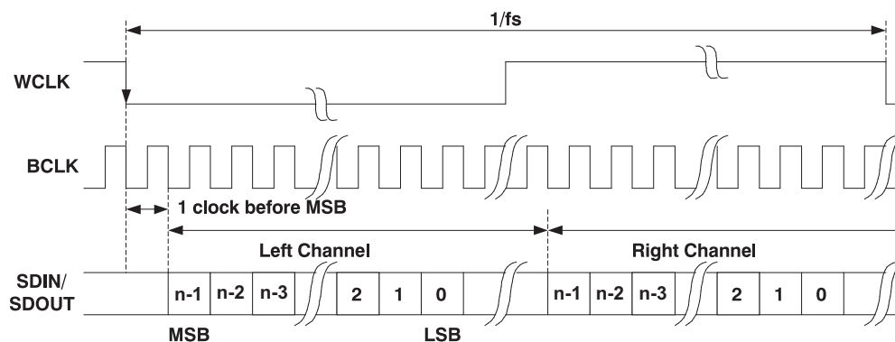
Figure 24. I 2 S Serial Data Bus Mode Operation
