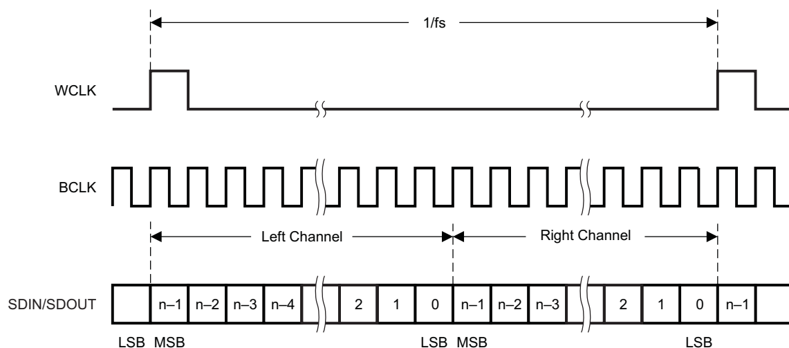
Figure 25. DSP Serial Bus Mode Operation
