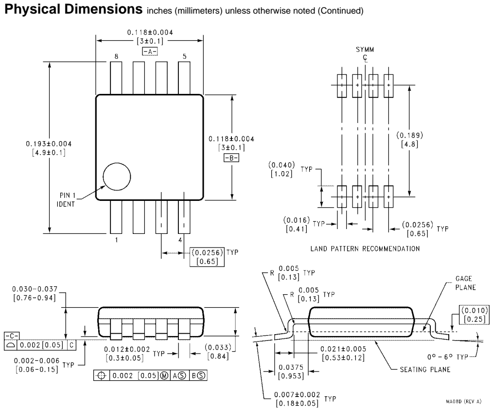
8-Lead Molded Small Outline Package (MSOP), JEDEC MO-187, 3.0mm Wide Package Number MA08D
