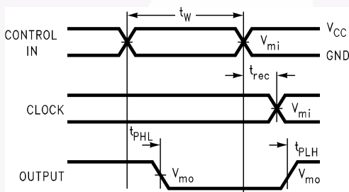
Propagation Delay, Pulse Width and t_{rec} Waveforms
