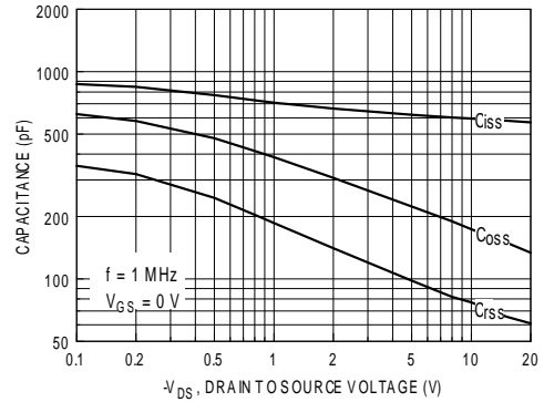
Figure 8. Capacitance Characteristics.
