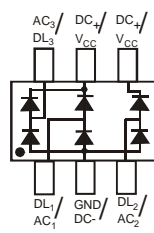
TOP VIEW Internal Schematic
