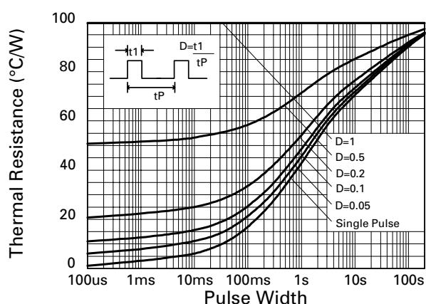
Transient Thermal Resistance Single Transistor "On"
