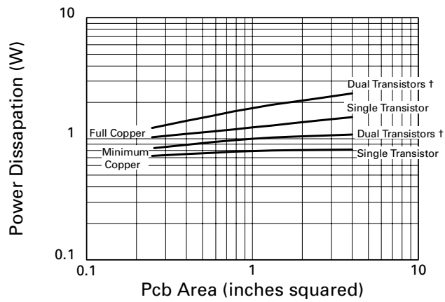
Pd v Pcb Area Comparison
