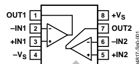
Figure 1. 8-Lead SOIC
