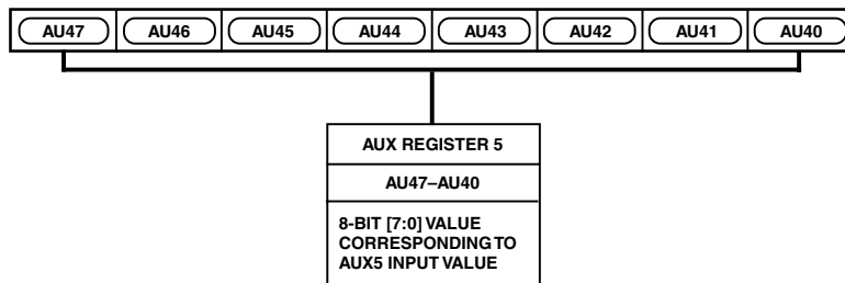
Figure 32. AUX Register 5
