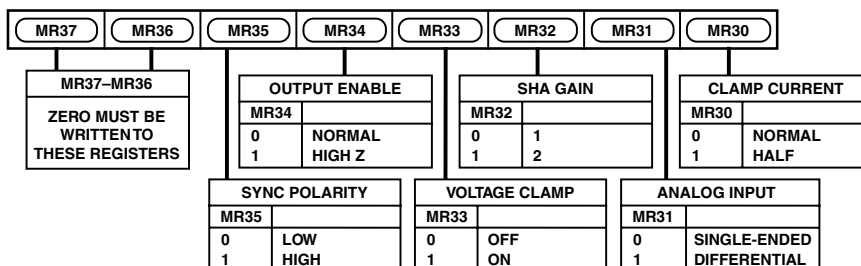
Figure 19. Mode Register 3
