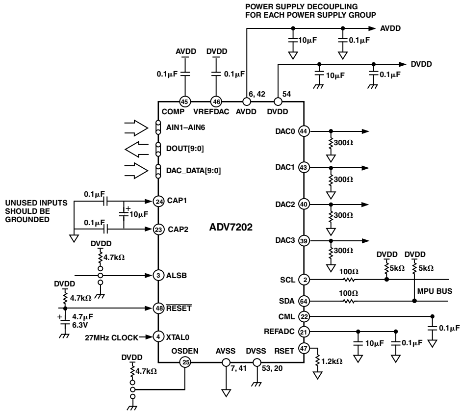
Figure 35. Suggested Schematic
