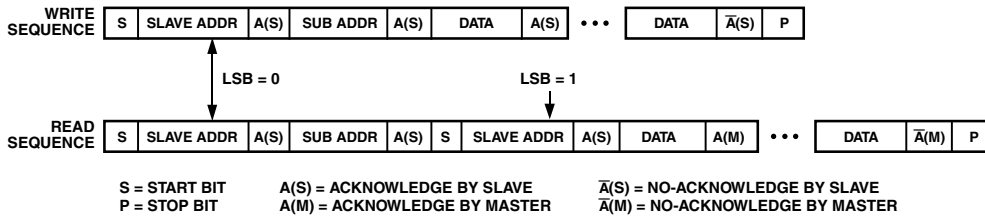
Figure 6. Write and Read Sequence
