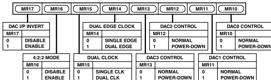
Figure 17. Mode Register 1
