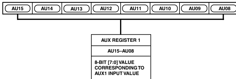
Figure 28. AUX Register 1
