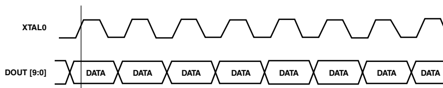
Figure 14. Standard Mode Digital Data O/P Format
