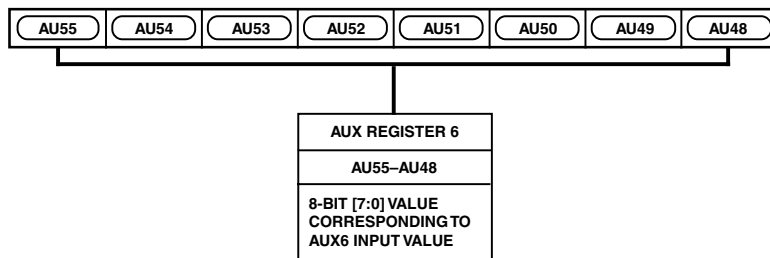
Figure 33. AUX Register 6
