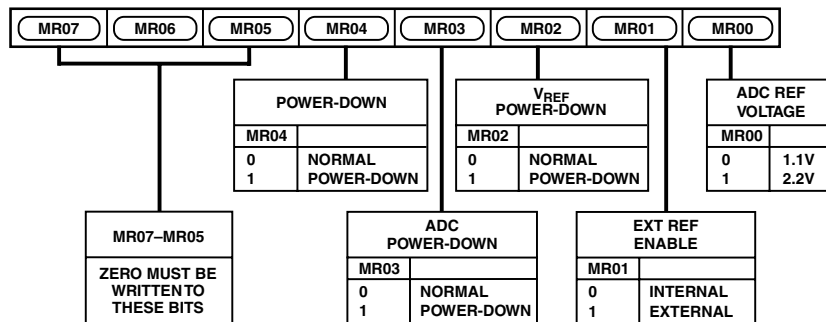
Figure 16. Mode Register 0
