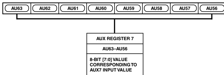
Figure 34. AUX Register 7
