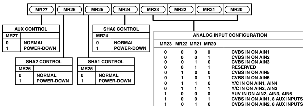
Figure 18. Mode Register 2
