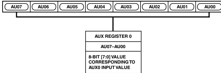
Figure 27. AUX Register 0
