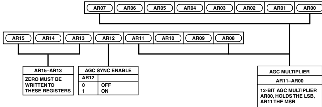
Figure 20. AGC Registers 0–1
