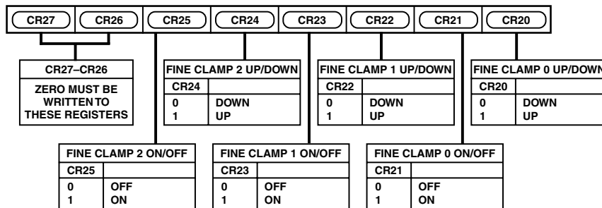
Figure 23. Clamp Register 2
