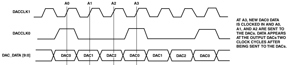
Figure 10. DAC Mode 1, Single Clock, Single Edge Input Data Format Timing Diagram*
