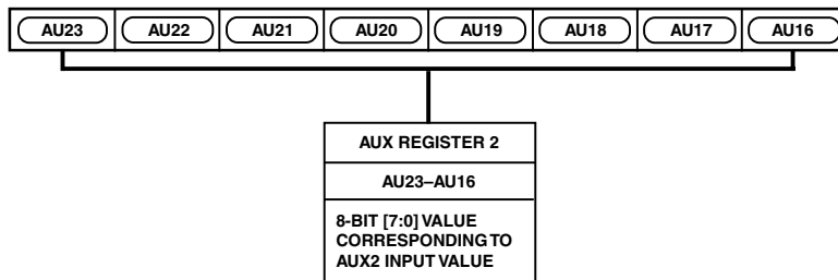
Figure 29. AUX Register 2
