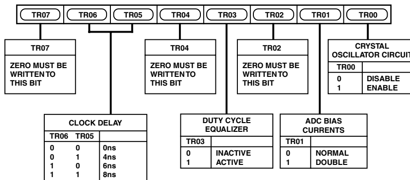
Figure 25. Timing Register 0
