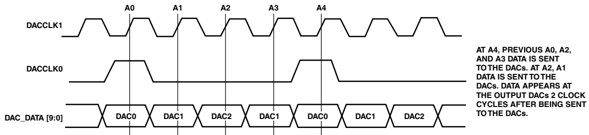
Figure 12. DAC Mode 3, 4:2:2 Input Data Format Timing Diagram
