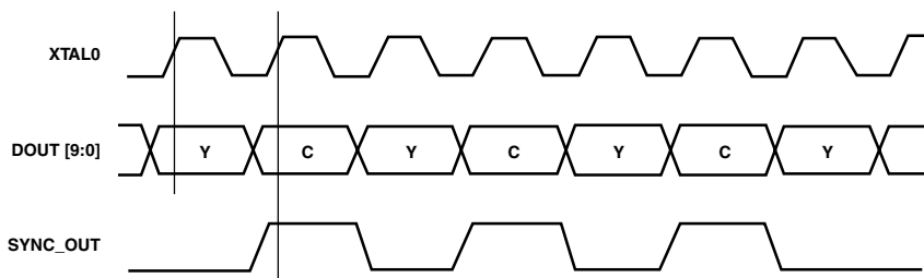
Figure 2. SYNC_OUT Output Timing, Y/C (S-VIDEO) Input
