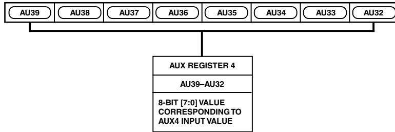
Figure 31. AUX Register 4
