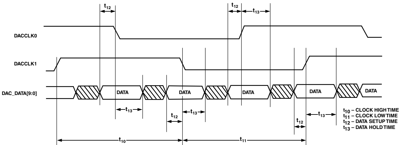
Figure 9. Input Data Format Timing Diagram Dual Clock
