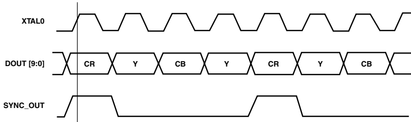
Figure 3. SYNC_OUT Output Timing, YCrCb Input
