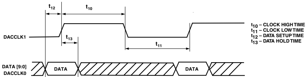
Figure 8. Input Data Format Timing Diagram Single Clock
