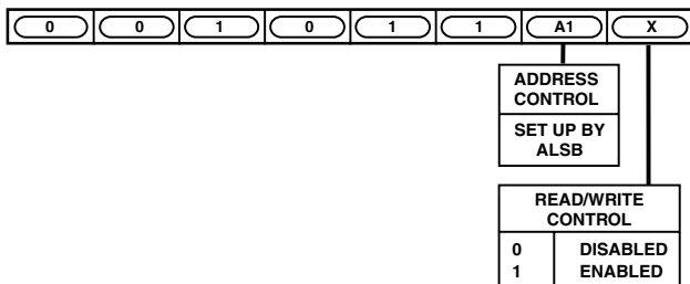
Figure 4. Slave Address
