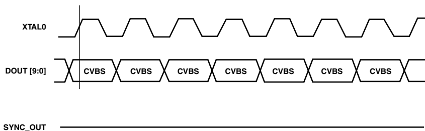
Figure 1. SYNC_OUT Output Timing, CVBS Input
