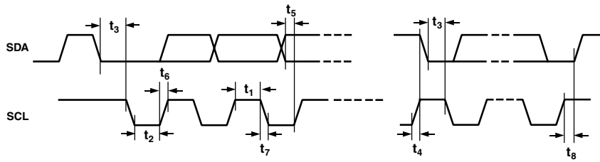
Figure 7. I 2 C MPU Port Timing Diagram
