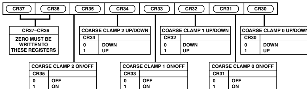
Figure 24. Clamp Register 3
