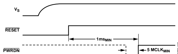
Figure 5. Power-Up Sequence for Tx Data Path
