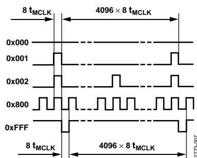
Figure 7. Σ-Δ Output Signals
