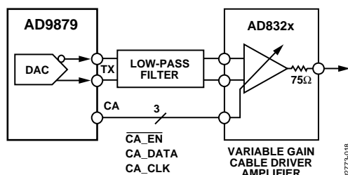
Figure 18. 16-Quadrature Modulation
