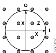
Figure 17. 16-Quadrature Modulation
