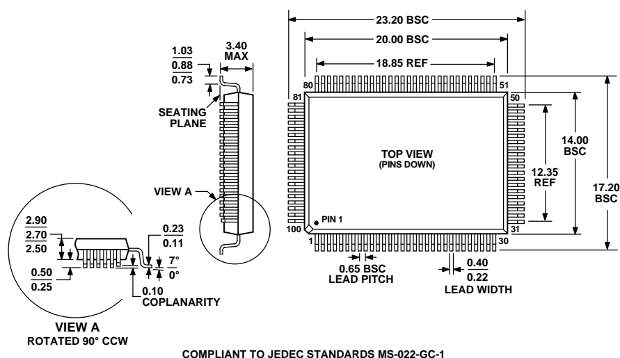
Figure 24. 100-Lead Metric Quad Flat Package [MQFP] (S-100-3) Dimensions shown in millimeters
