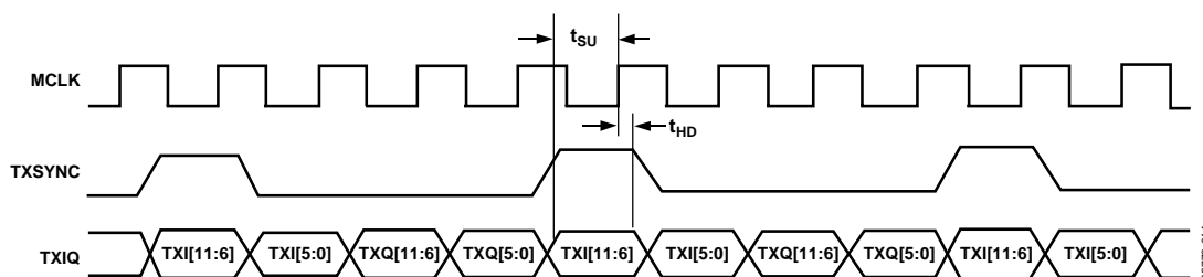
Figure 14. Transmit Path Timing
