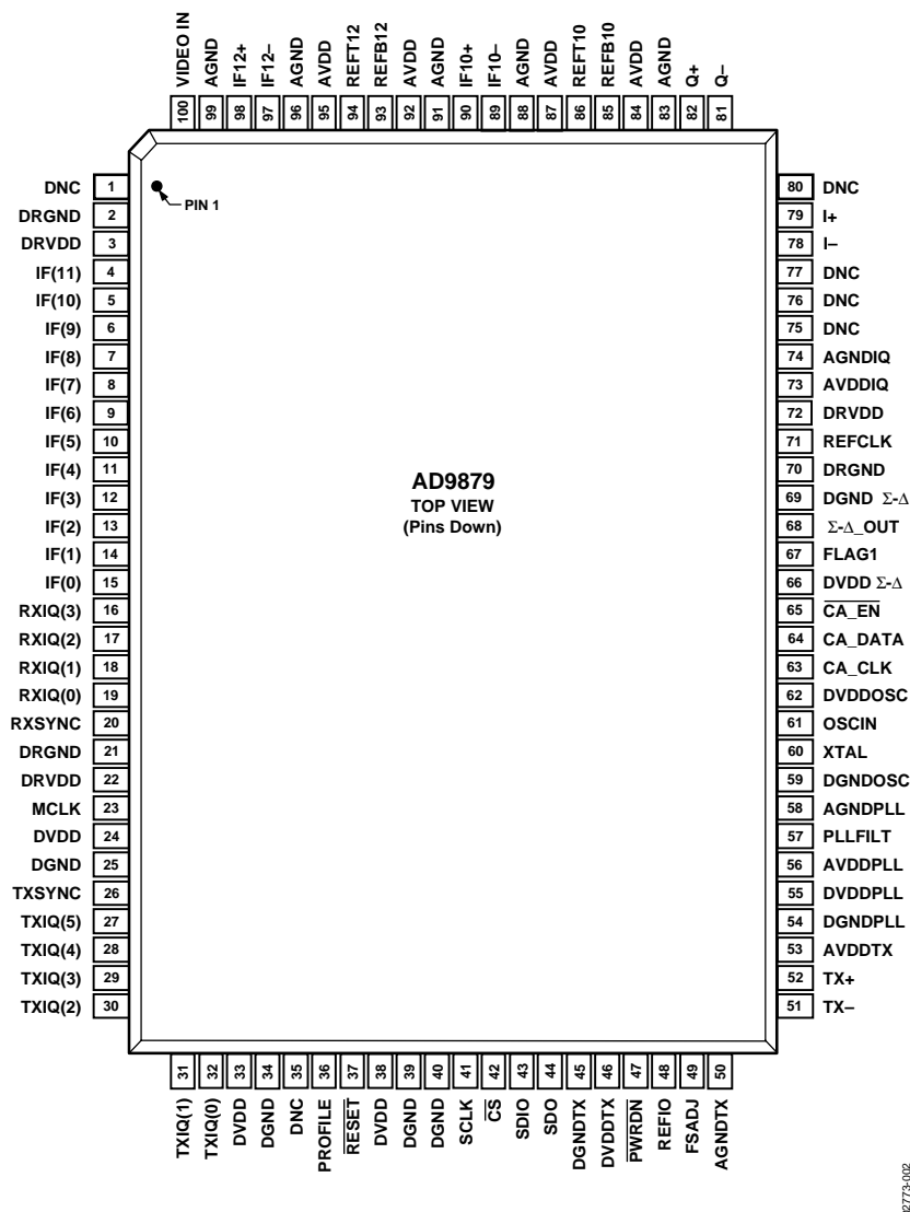
Figure 2. Pin Configuration
