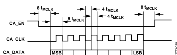
Figure 20. Cable Amplifier Interface Timing
