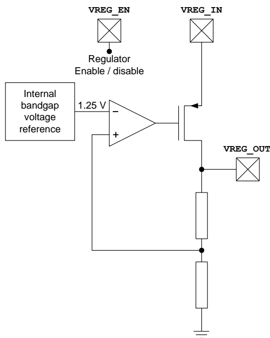
Figure 28. Voltage regulator, simplified schematic
