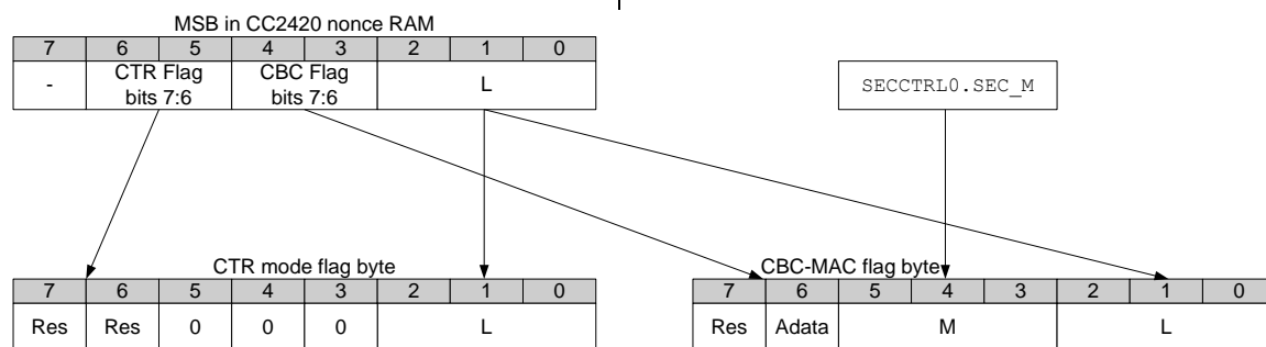
Figure 26. CC2420 Security Flag Byte
